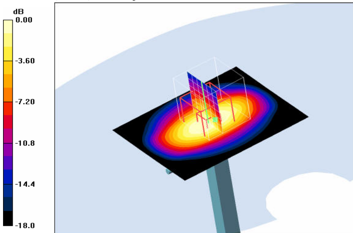
0 dB = 42.5mW/g
