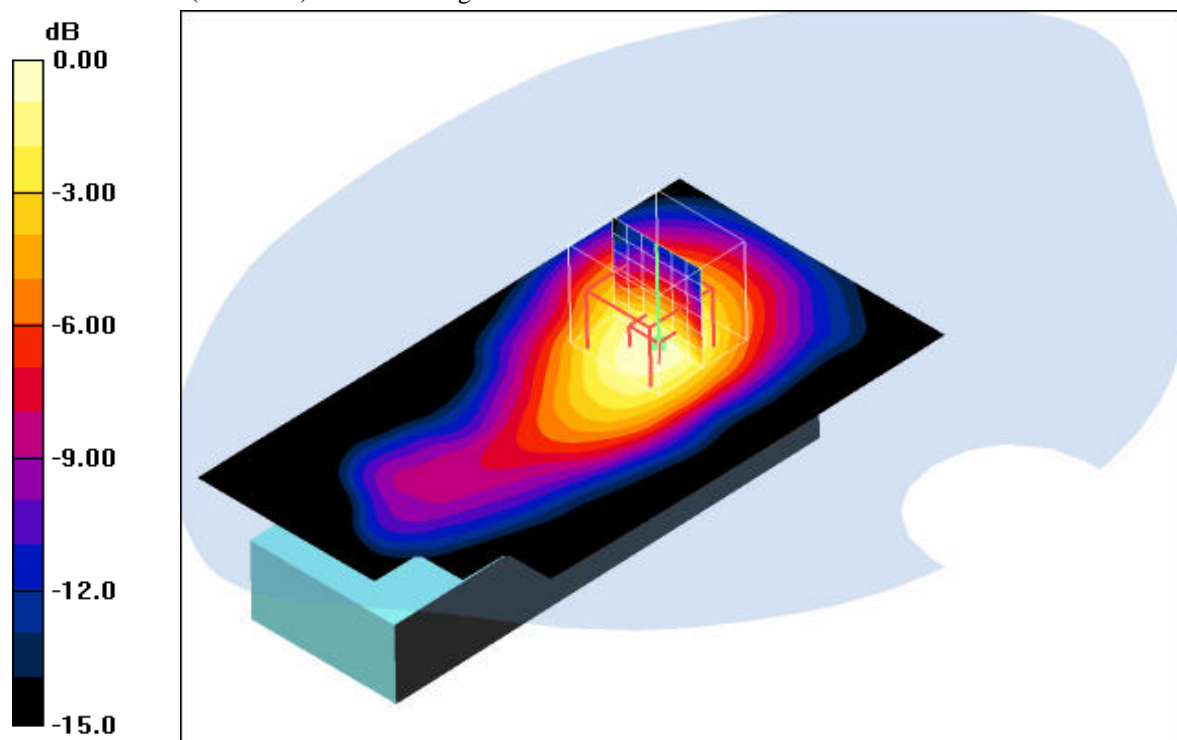
0 dB = 0.047mW/g
