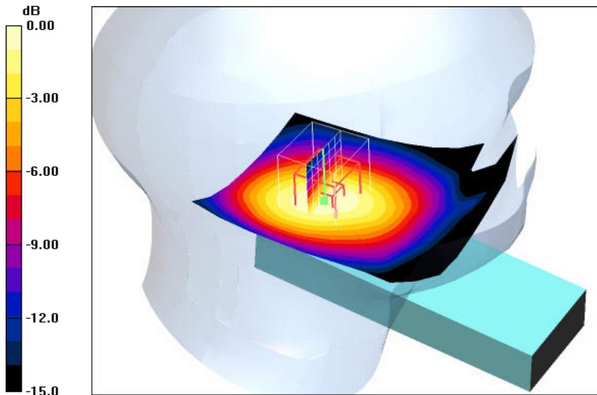
0 dB = 0.024mW/g
