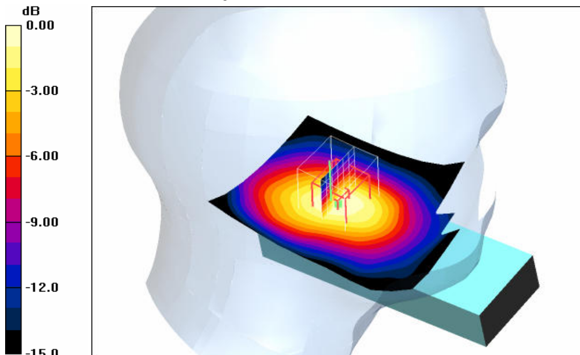
0 dB = 0.046mW/g
