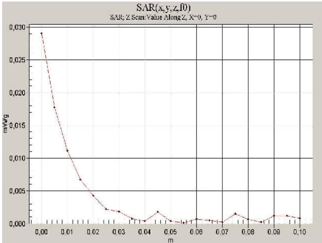
Photo 25: Z-axis scans 1900 MHz body
