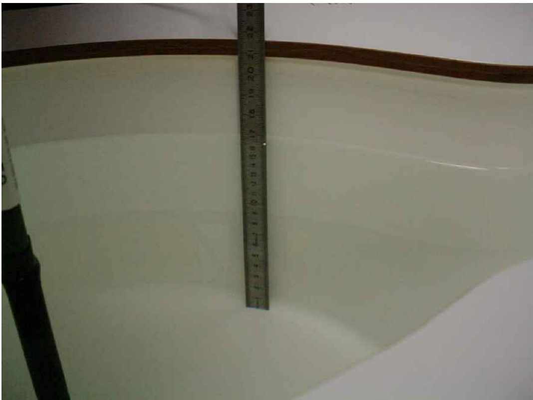
Photo 23: Liquid depth 1900 MHz body simulating liquid
