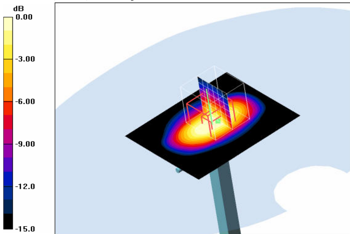
0 dB = 44.1mW/g
