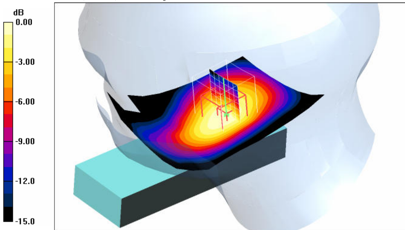
0 dB = 0.040mW/g
