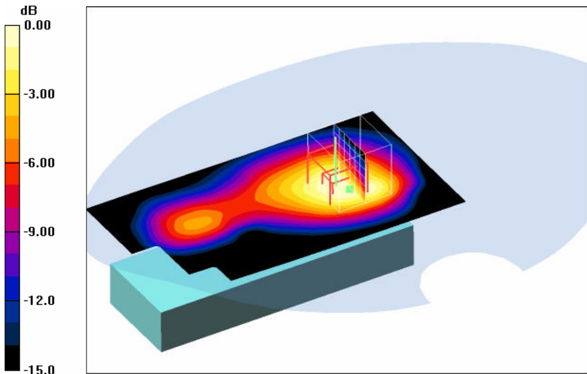
0 dB = 0.050mW/g
