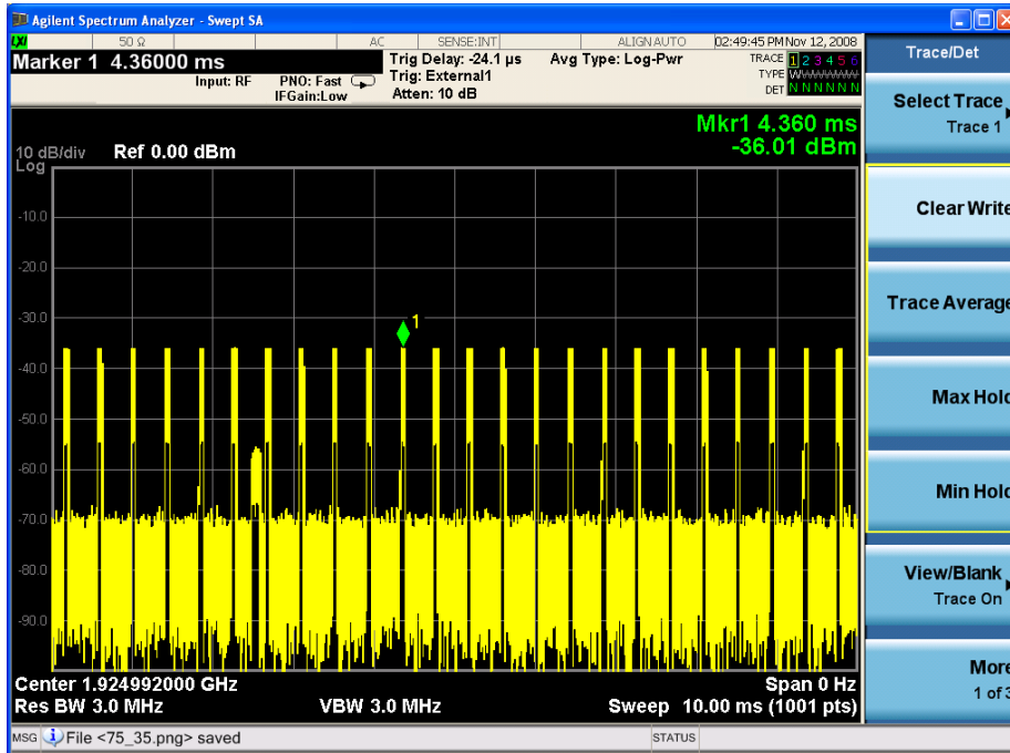
50 μs Pulses
