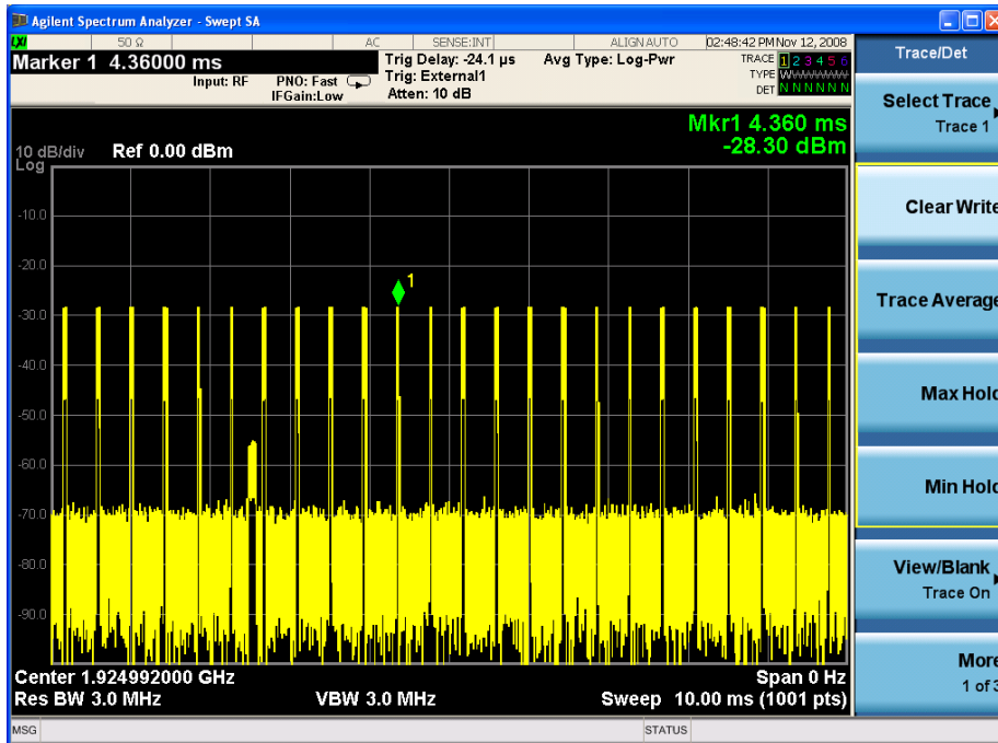
35 μs Pulses
