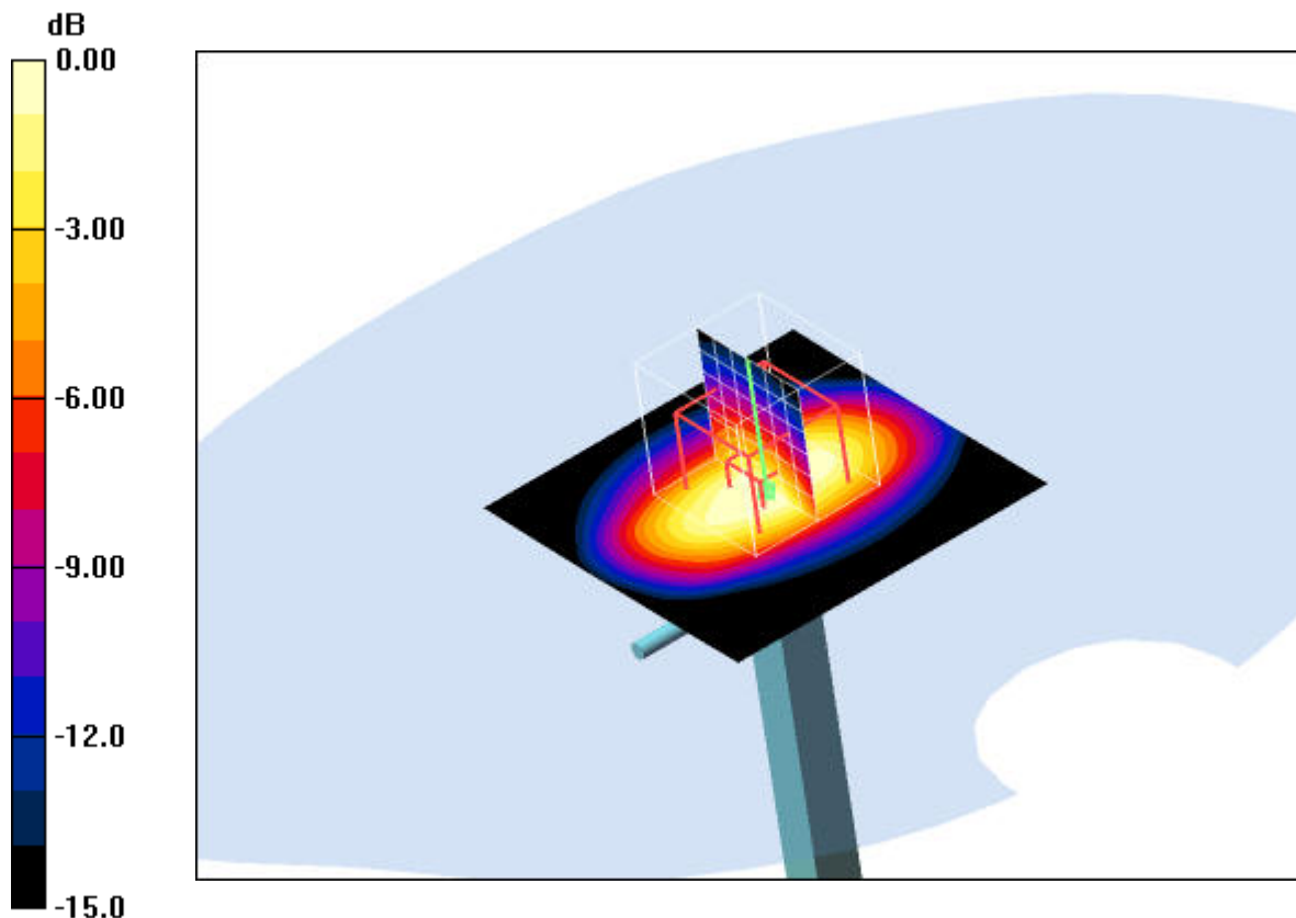
0 dB = 42.6mW/g
