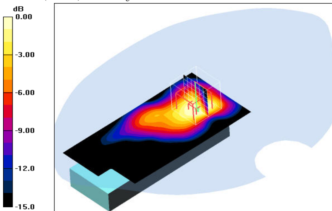
0 dB = 0.060mW/g
