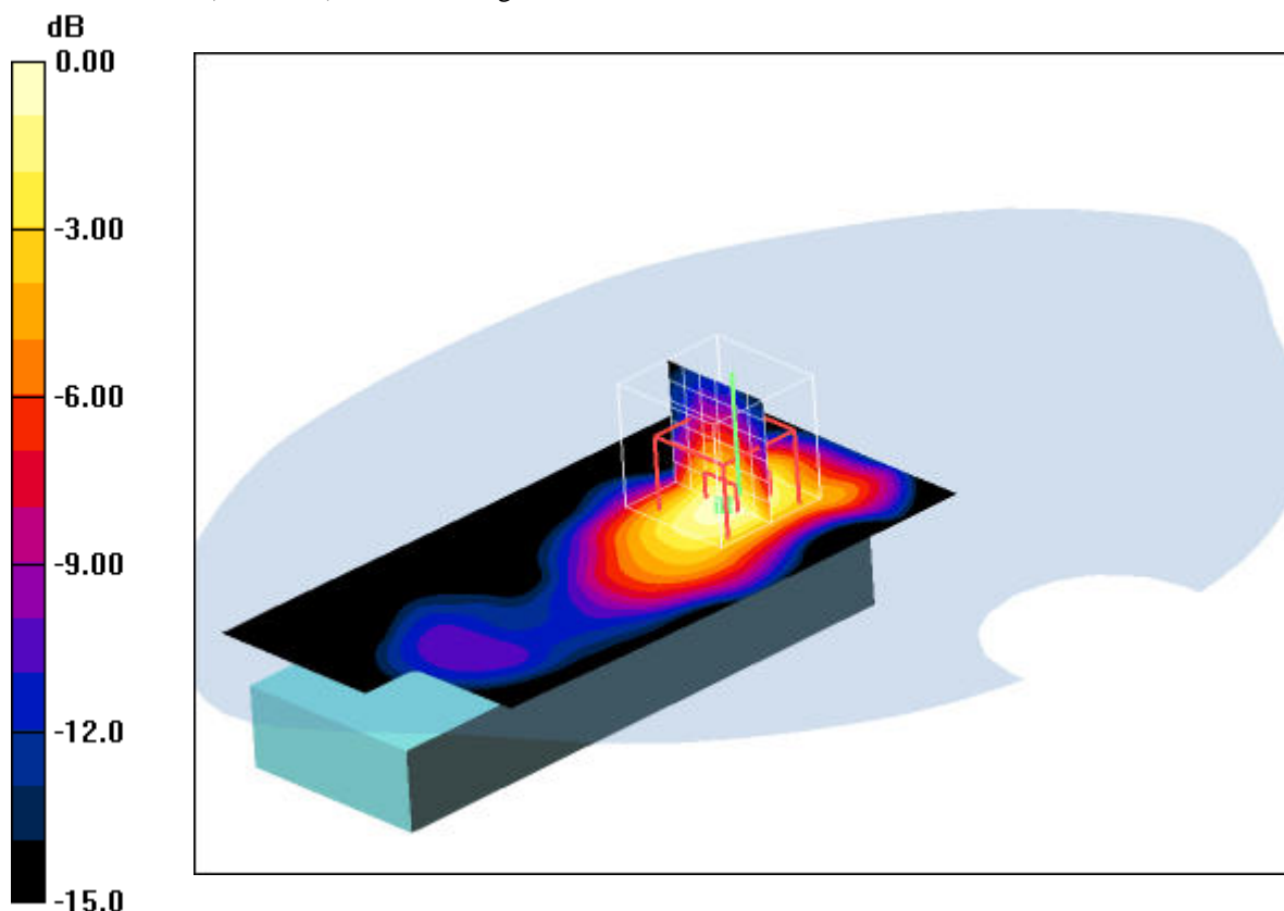
0 dB = 0.039mW/g
