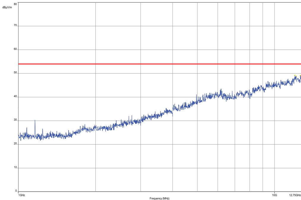
Plot 3: 1 GHz to 12.75 GHz, RX mode, vertical & horizontal polarization
