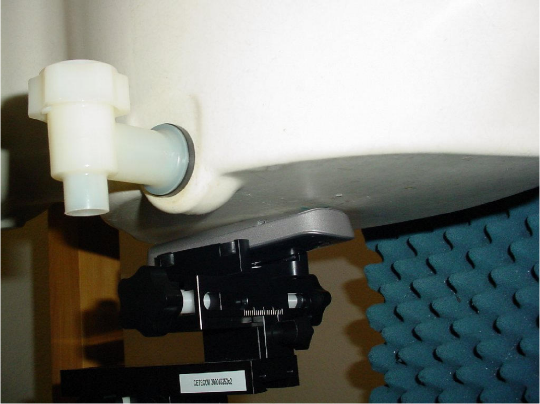
Photo 23: Test position body worn rear side without any distance and clip
