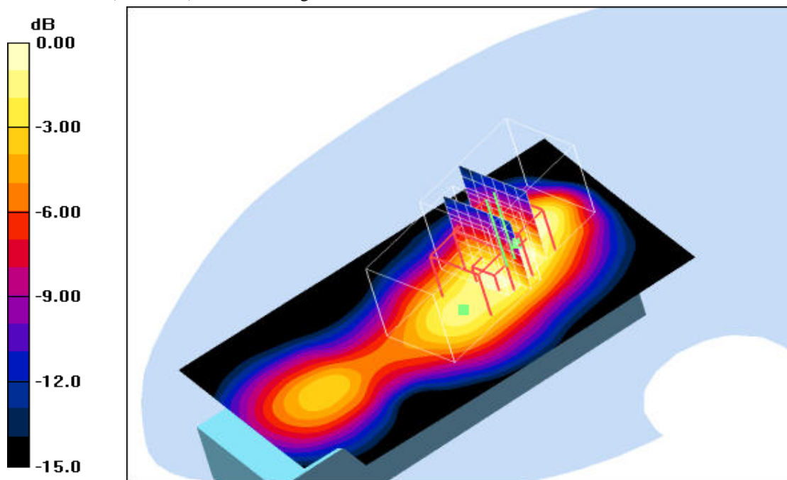
0 dB = 0.046mW/g
