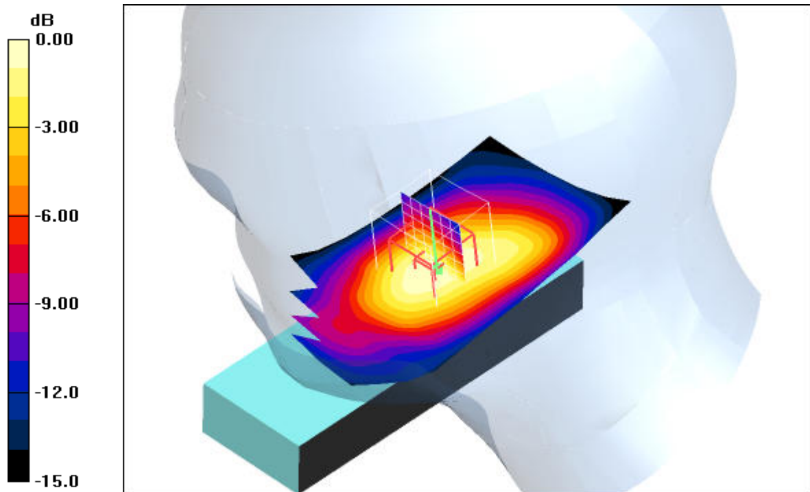
0 dB = 0.048mW/g
