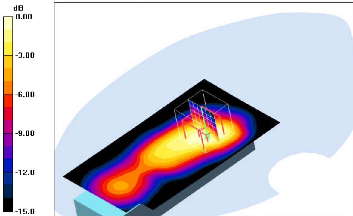
0 dB = 0.056mW/g
