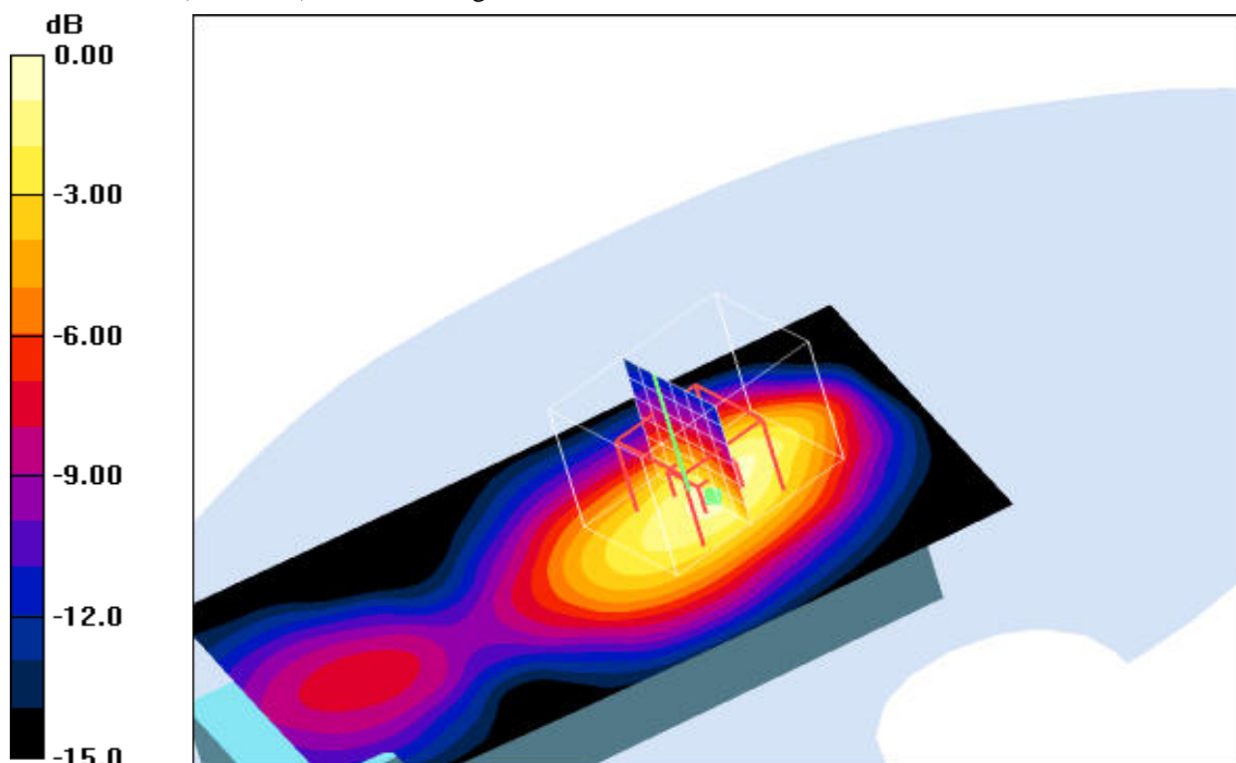
0 dB = 0.042mW/g
