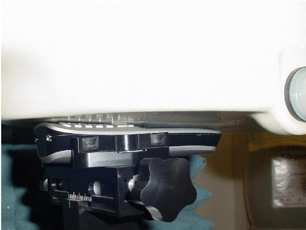
Photo 18: Test position body worn front side without any distance
