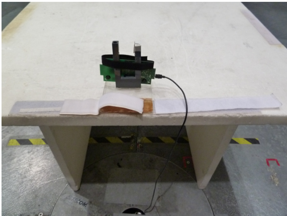
Photo 2: Radiated Emission
