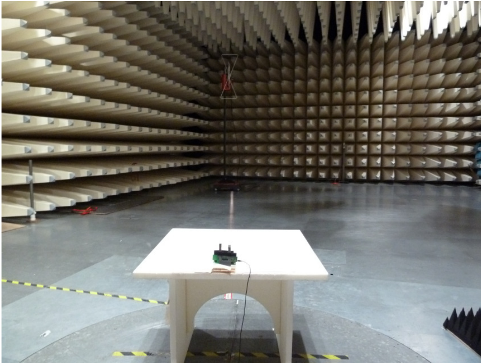
Photo 3: Radiated Emission
