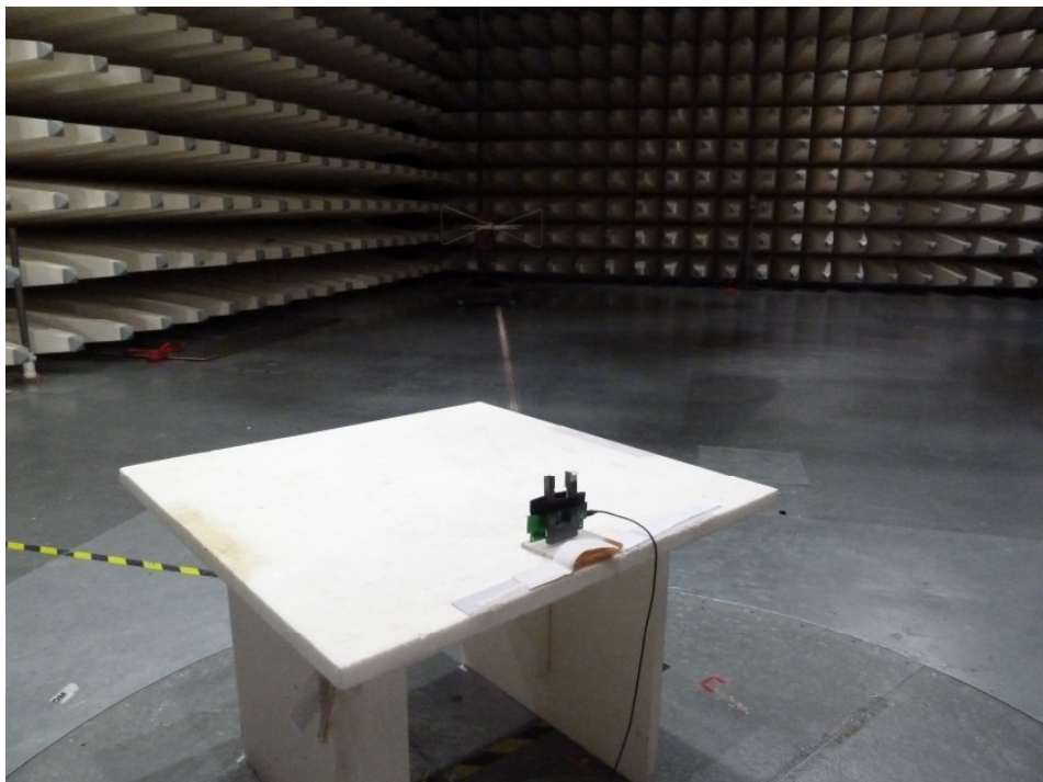
Photo 2: Radiated Emission
