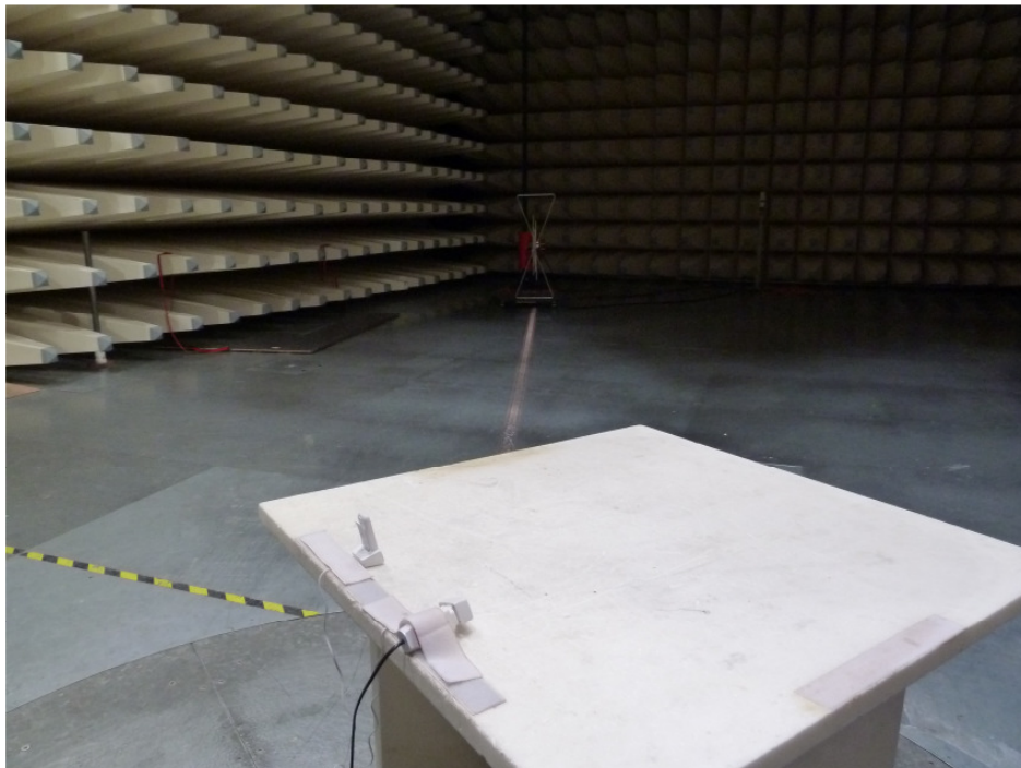
Photo 2: Radiated Emission
