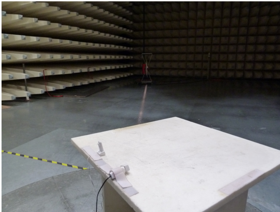
Photo 2: Radiated Emission
