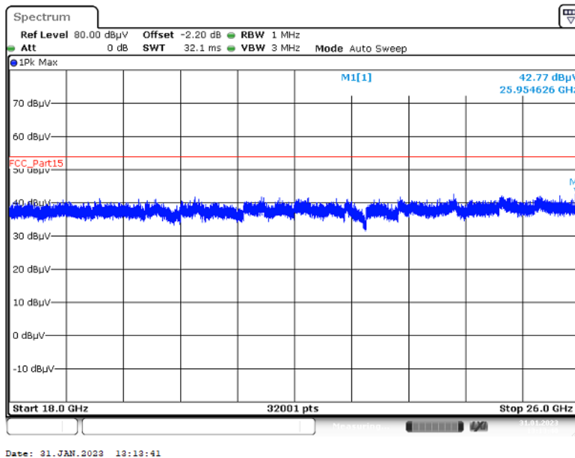
Plot 4: 18 GHz to 26 GHz, TX mode, valid for all channels, vertical & horizontal polarization, 1 Msp
