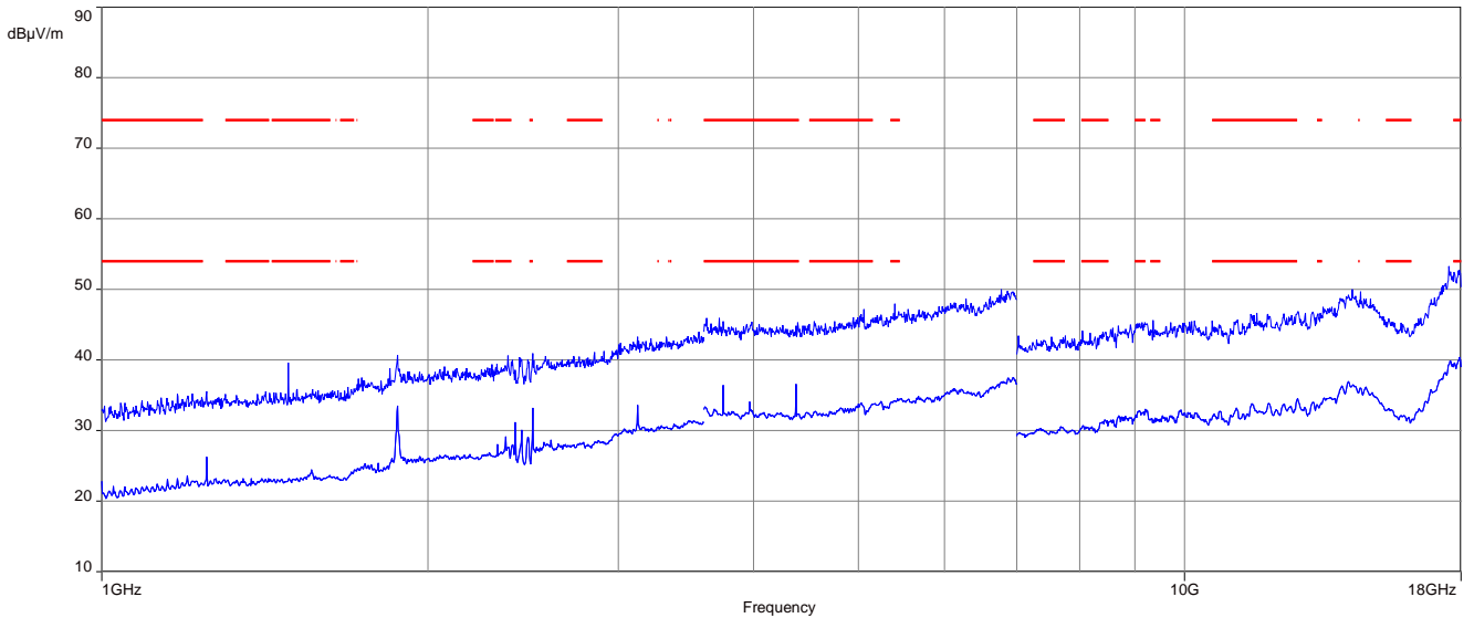
Plot 3: 1 GHz to 18 GHz, TX mode, 2480 MHz, vertical & horizontal polarization, 1 Msp
