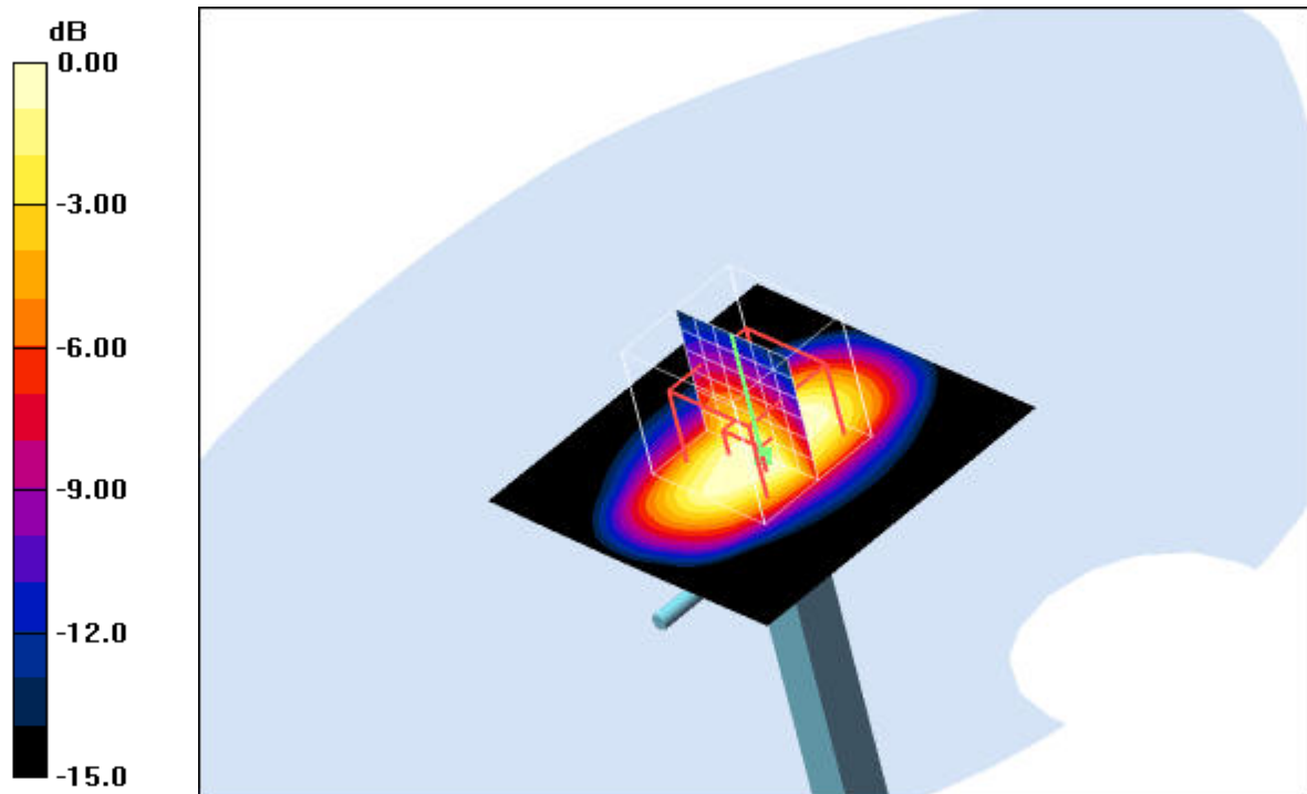
0 dB = 44.2mW/g
