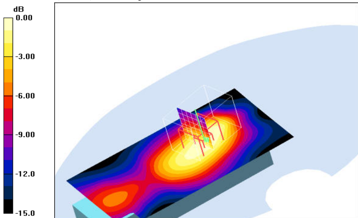
0 dB = 0.024mW/g
