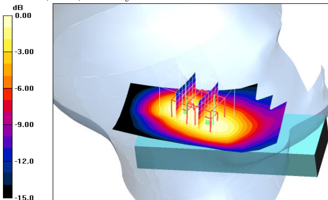
0 dB = 0.034mW/g
