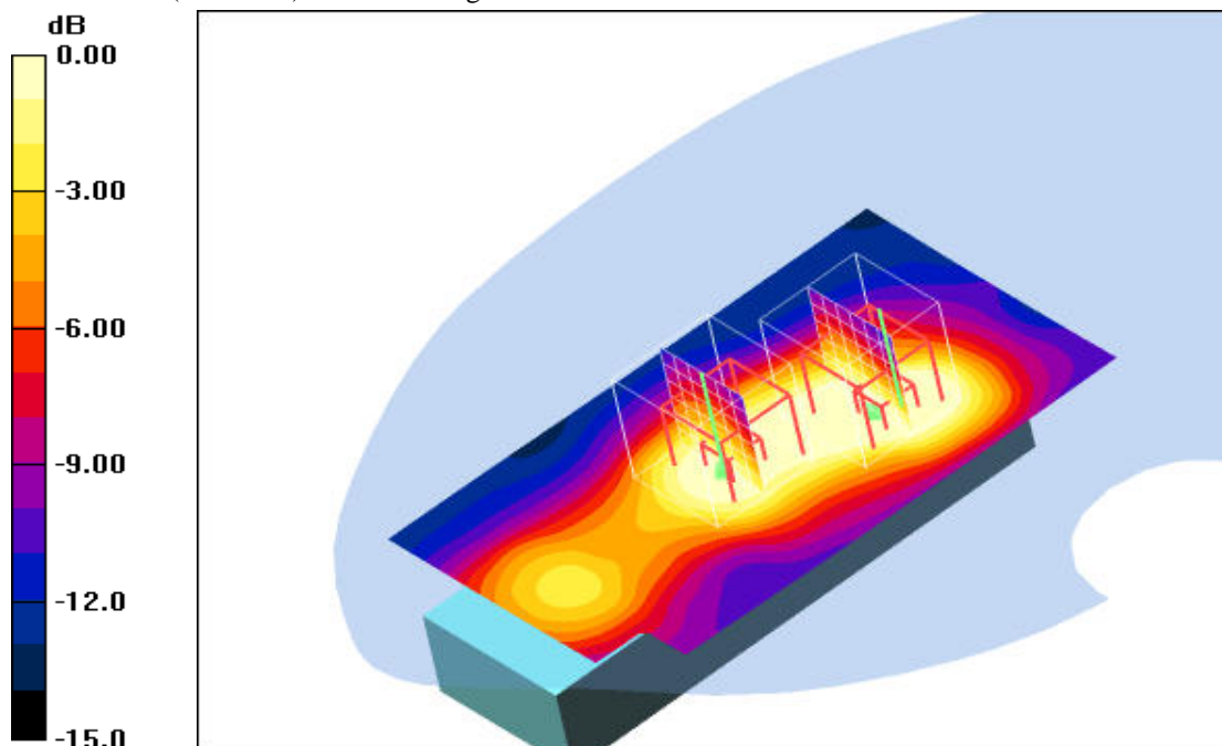
0 dB = 0.033mW/g
