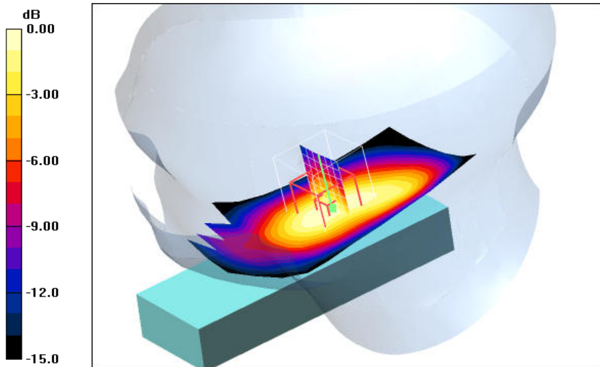
0 dB = 0.035mW/g
