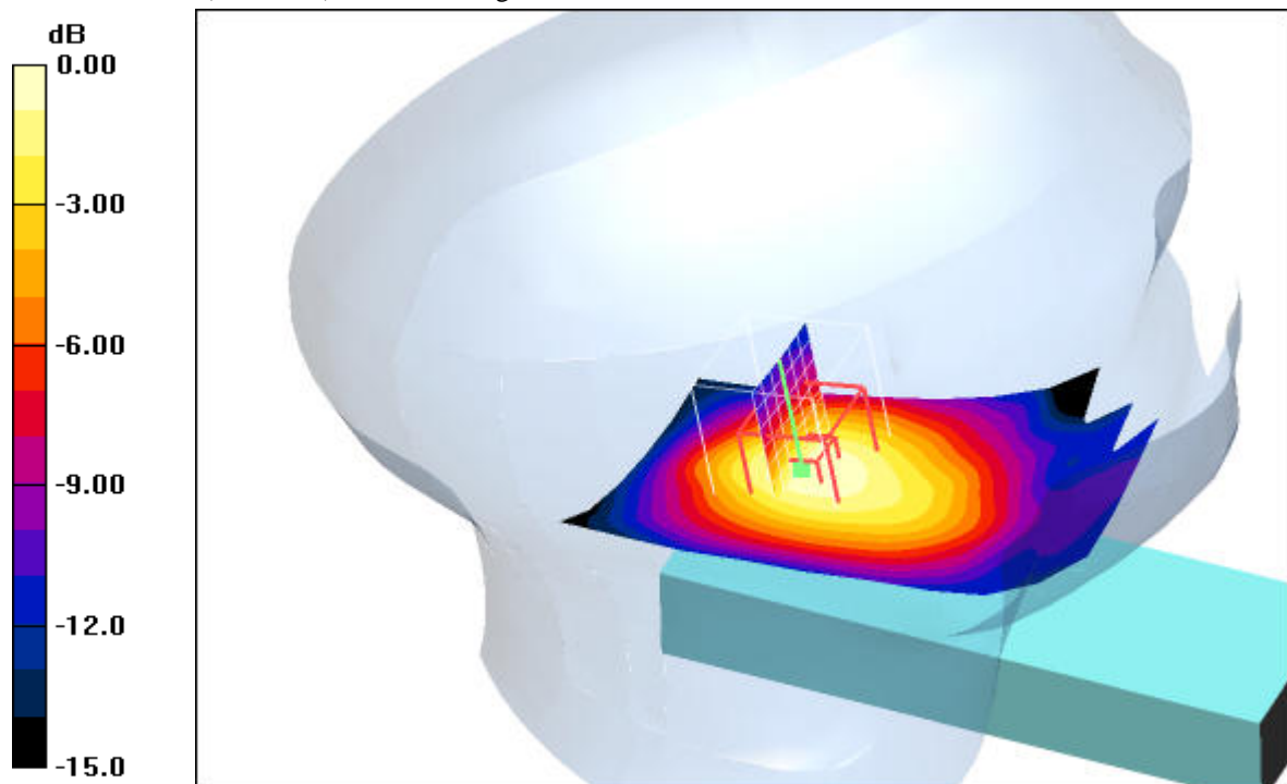
0 dB = 0.022mW/g
