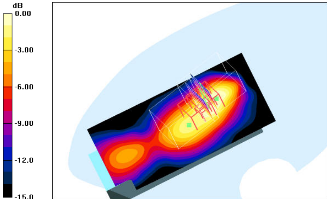
0 dB = 0.031mW/g
