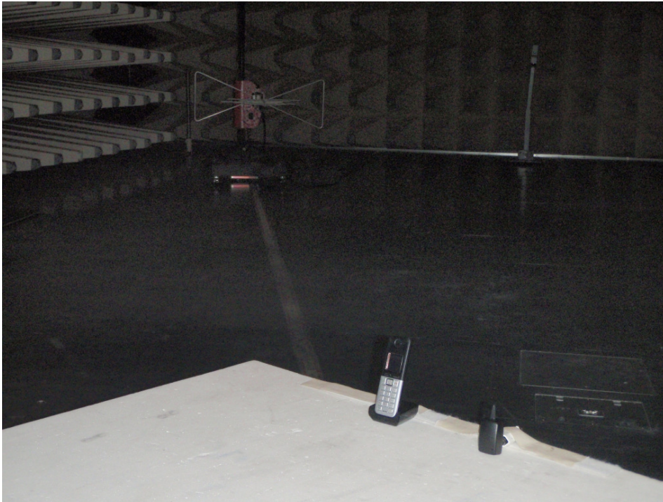
Photo 3: Radiated Emission
