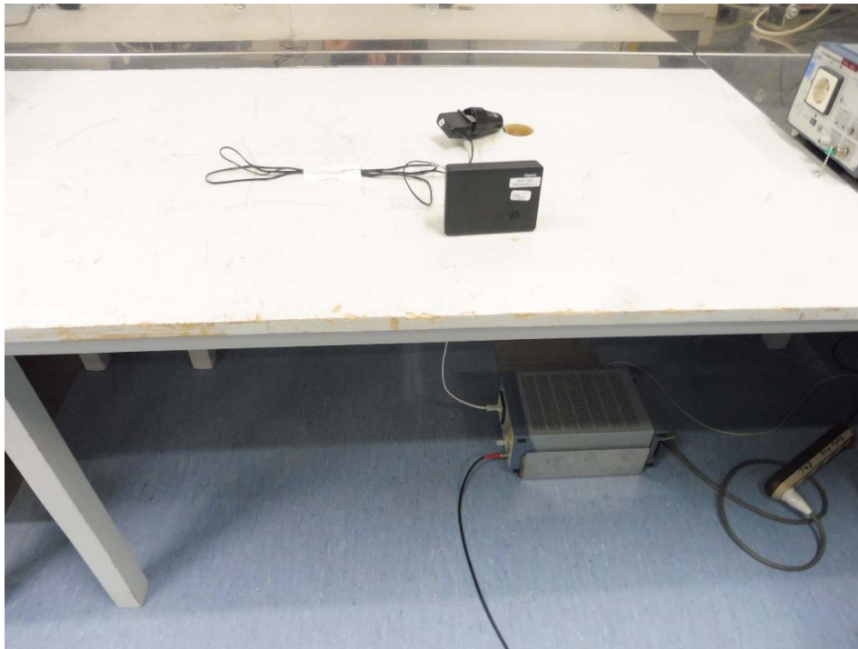
Photo 3: Conducted Emission
