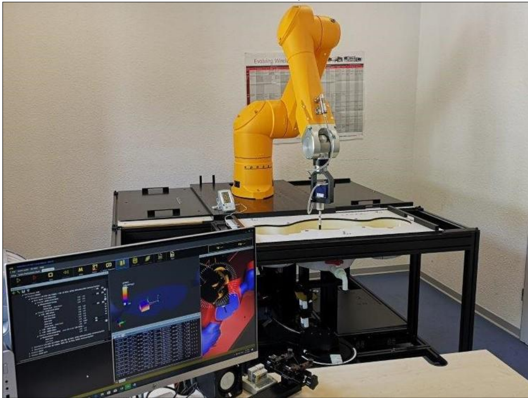
Photo 1: Measurement System DASY 6
