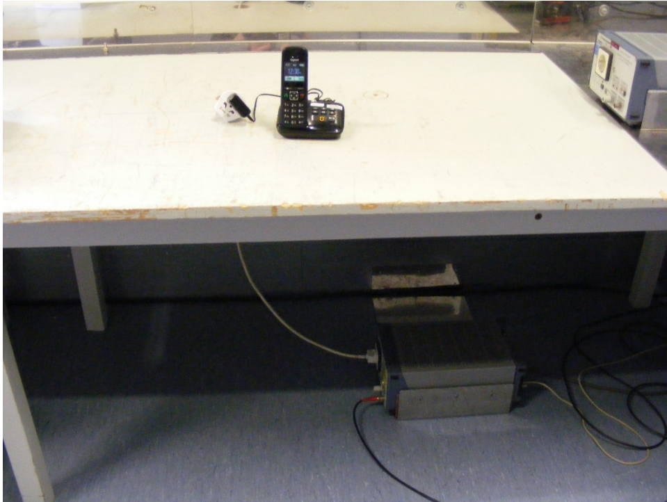
Photo 3: Conducted Emission
