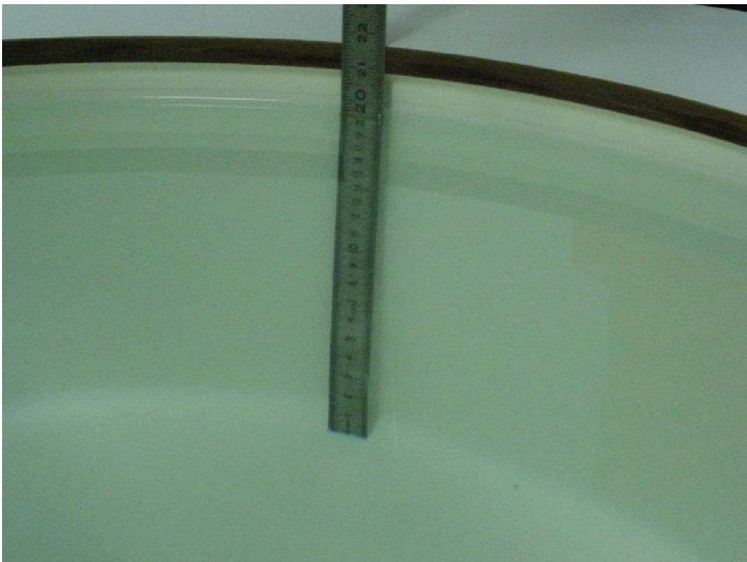
Photo 21: Liquid depth 1900 MHz body simulating liquid
