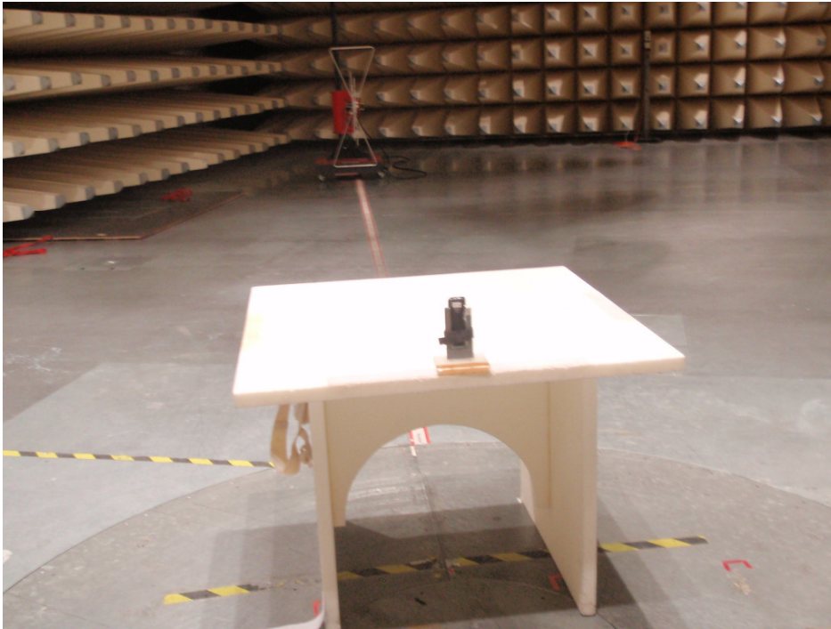
Photo 3: Radiated Emission
