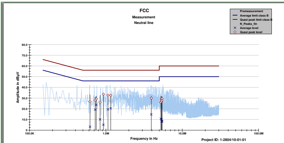
Idle mode, neutral line
