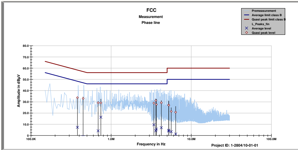
Idle mode, phase line
