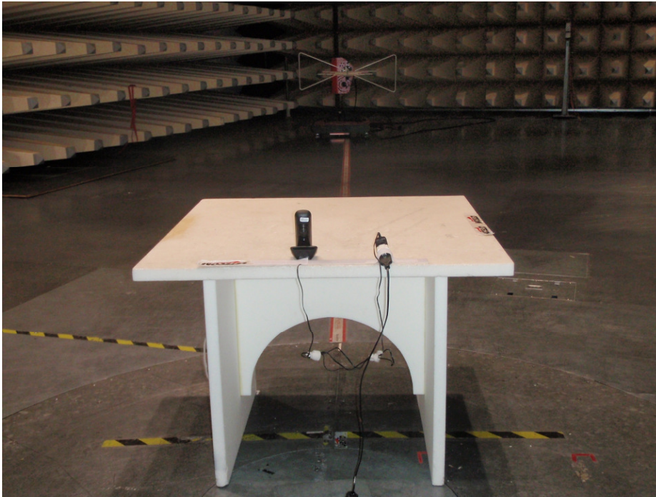
Photo 3: Radiated Emission
