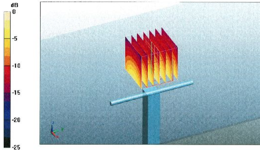
0 dB = 12.9mW/g
