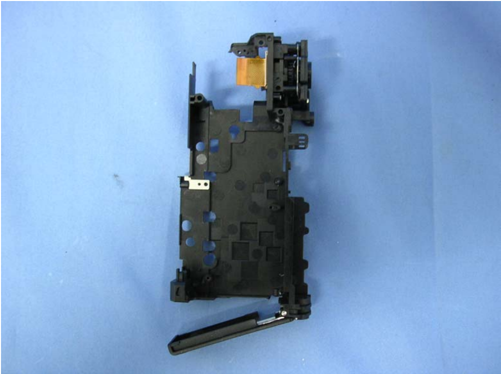
(42) EUT Photo
