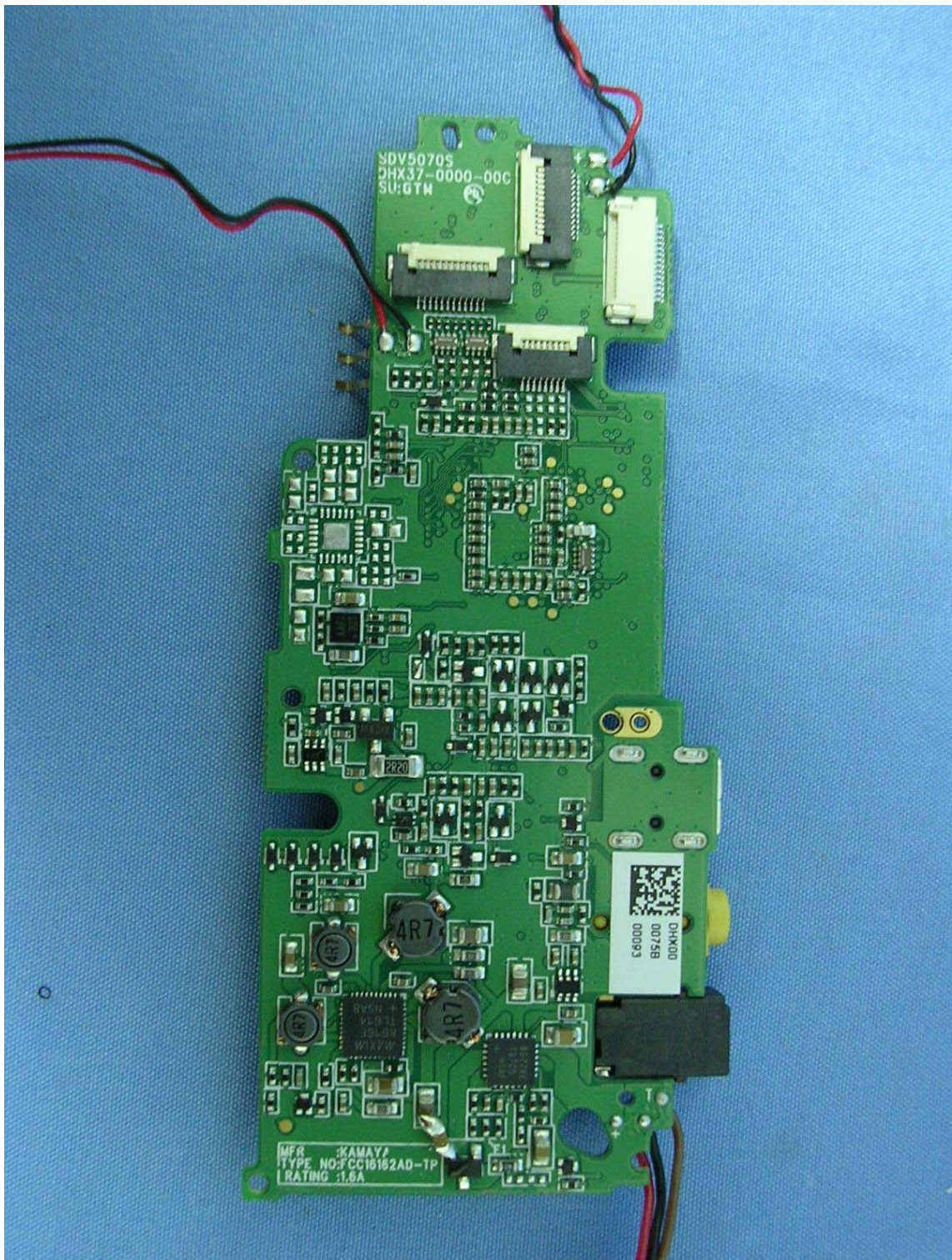
(38) EUT Photo
