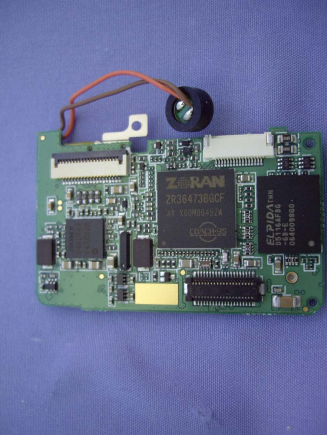
(45) EUT Photo
