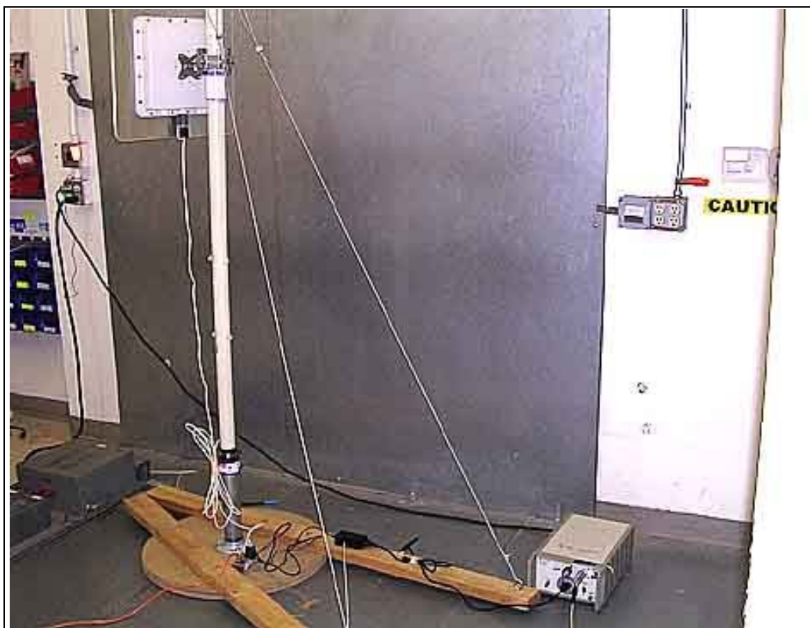
FCC 15.107 Mains Conducted Emissions - Back View - 58-AE-26F
