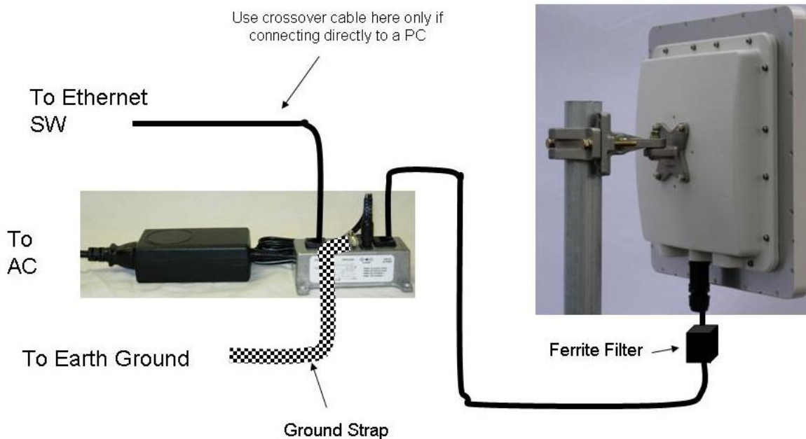
Figure 1 Connection Diagram
