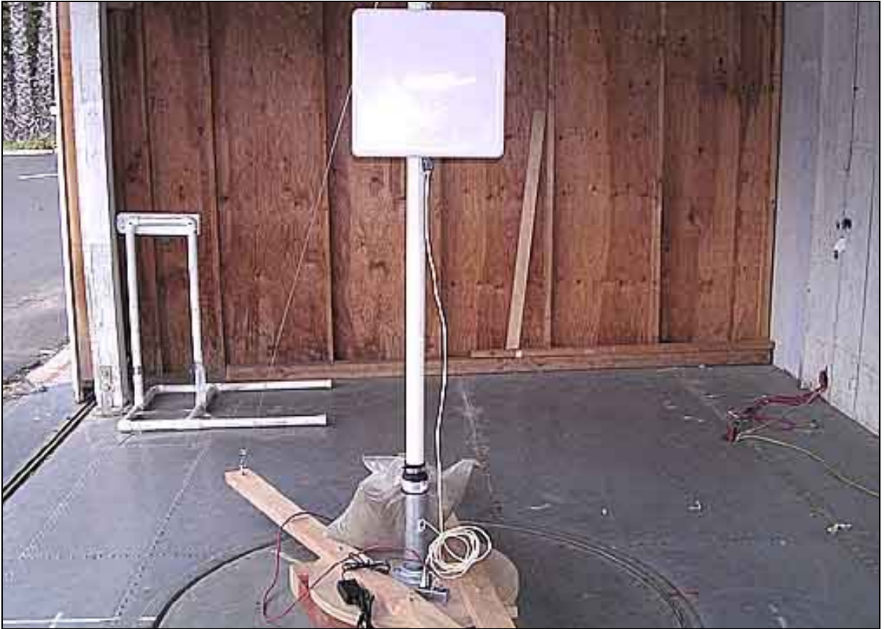
FCC 15.109 Radiated Emissions - Back View - 24-AE-19F
