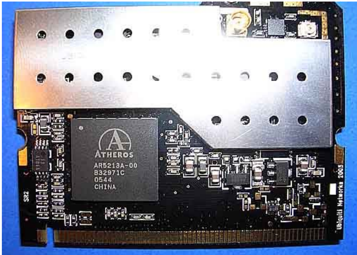
2420S Transmitter Board Top
