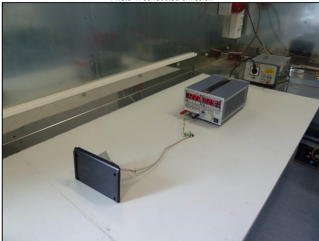
Photo 1: conducted emission
