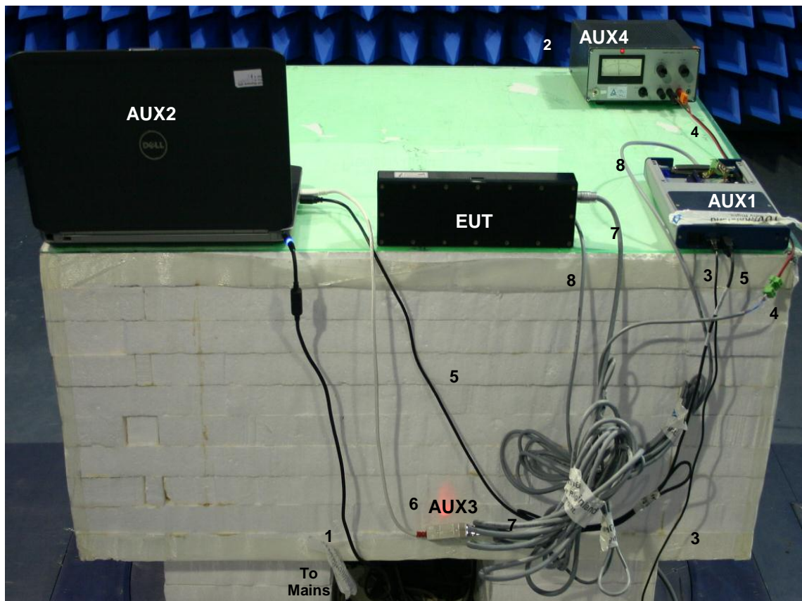
Photo 1: basic setup
