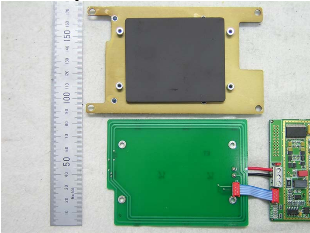
PCB Antenna Bottom View
