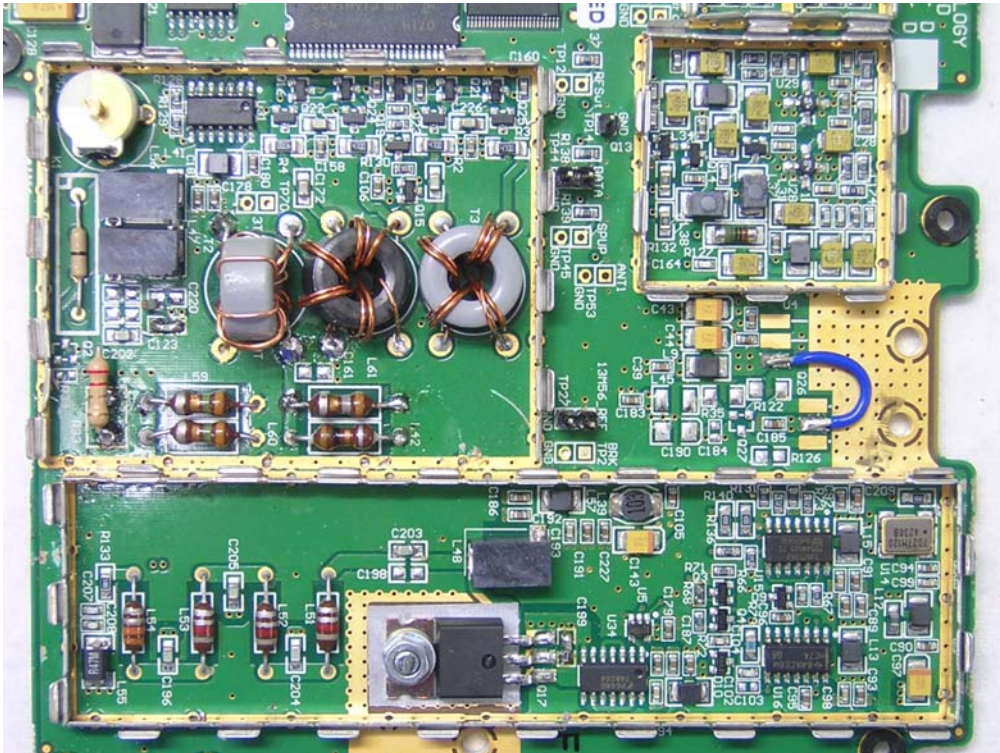
PCB RF Section
