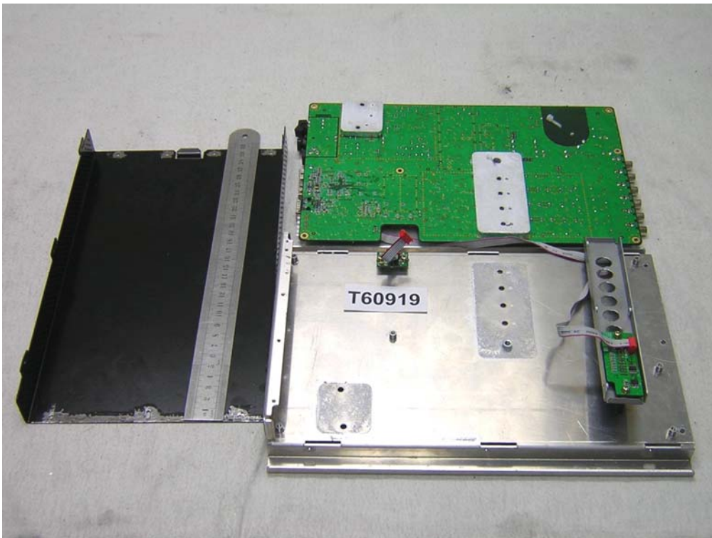
Exploded View 2
