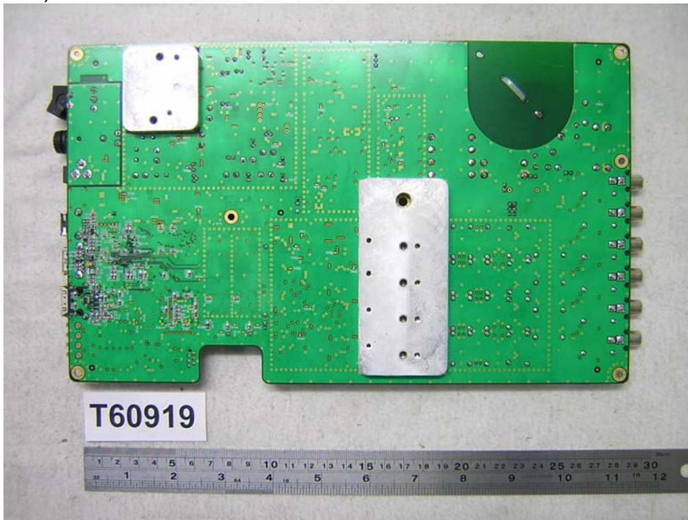
Mains Board, Bottom View
