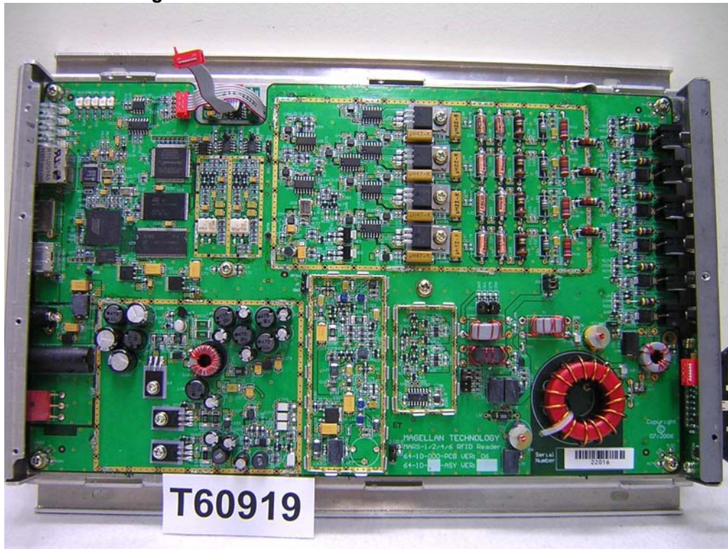
Main Board No Shielding Cans
