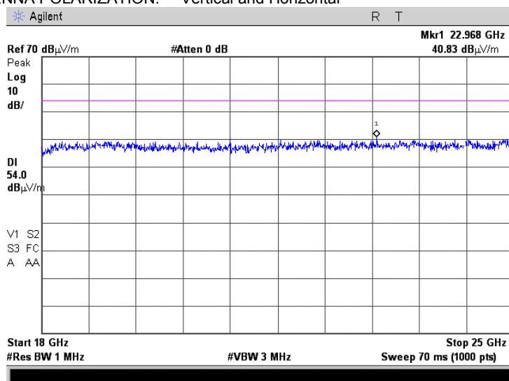
Plot 7.3.29 Radiated emission measurements from 18000 to 25000 MHz at the mid carrier frequency
