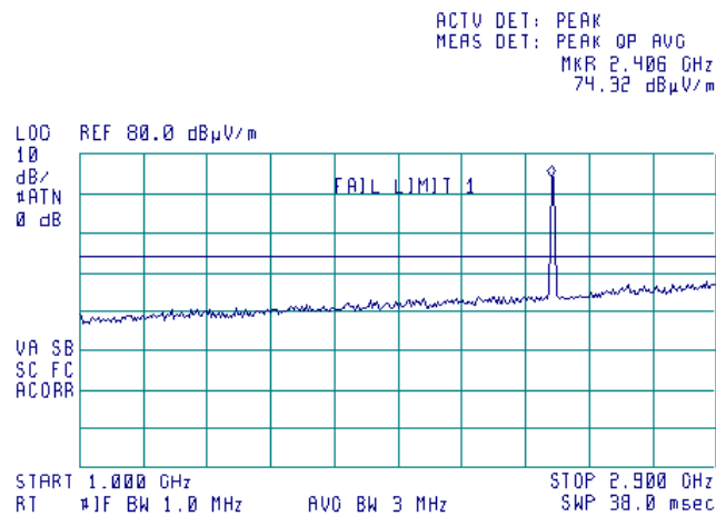
Plot 7.3.15 Radiated emission measurements from 1000 to 2900 MHz at the high carrier frequency
