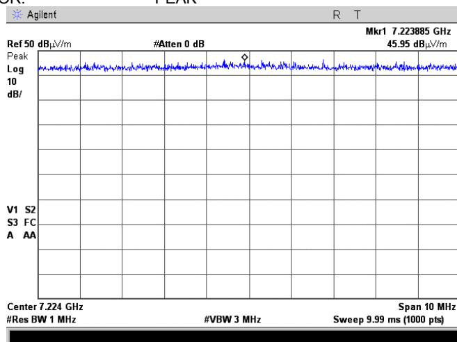
Plot 7.3.36 Radiated emission measurements at the third harmonic of high carrier frequency
