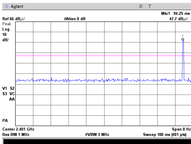
Plot 7.3.50 Transmission pulse duration within 100 msec
