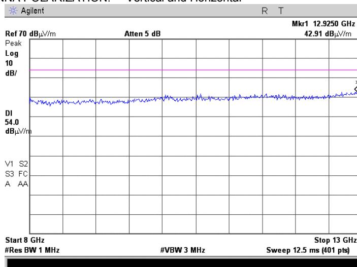
Plot 7.3.23 Radiated emission measurements from 8000 to 13000 MHz at the mid carrier frequency
