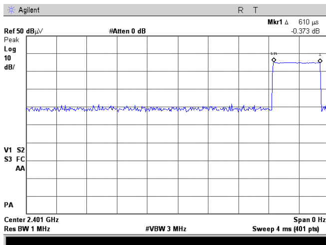
Plot 7.3.49 Transmission pulse duration within 100 msec
