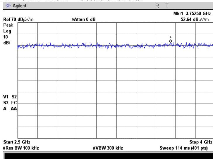
Plot 7.3.17 Radiated emission measurements from 2900 to 4000 MHz at the mid carrier frequency
