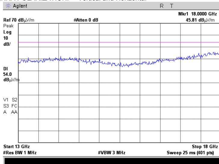
Plot 7.3.27 Radiated emission measurements from 13000 to 18000 MHz at the high carrier frequency
