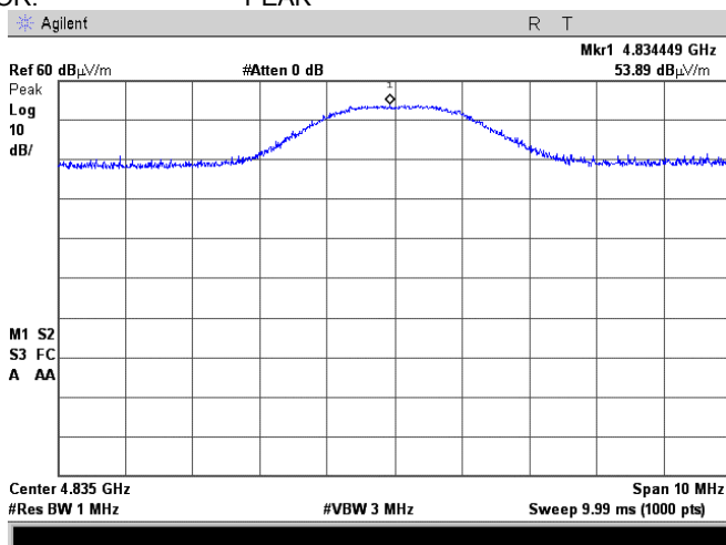
Plot 7.3.34 Radiated emission measurements at the third harmonic of low carrier frequency
