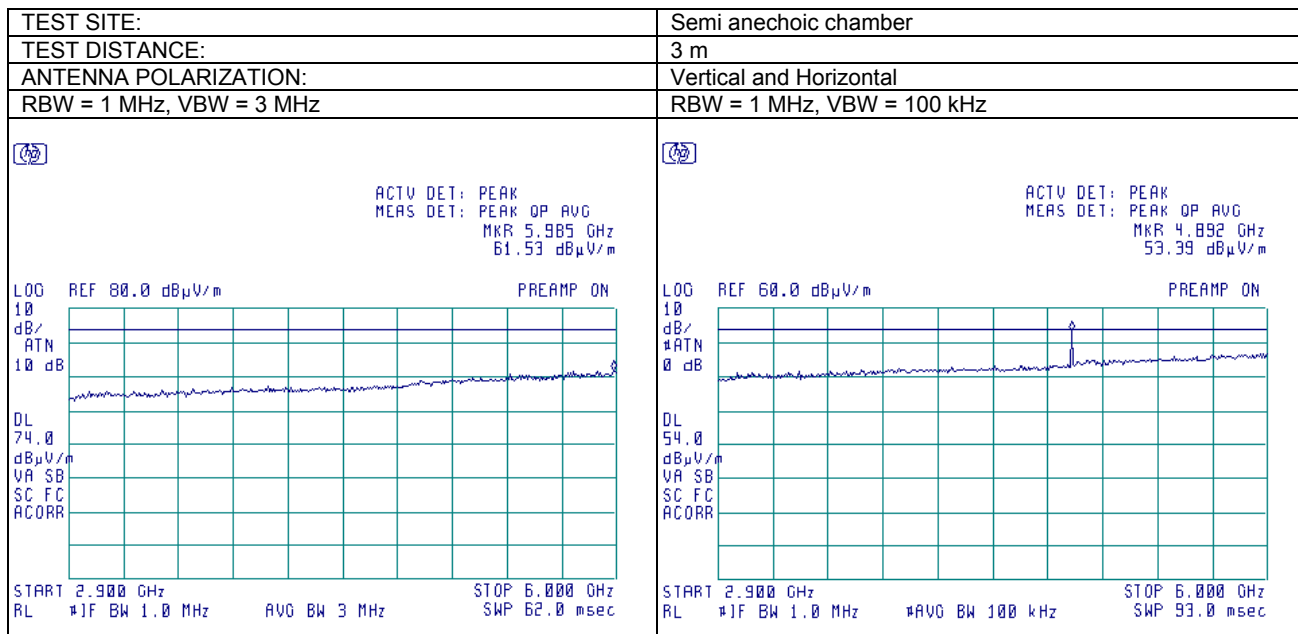
Plot 7.3.23 Radiated emission measurements from 2900 to 6000 MHz at the mid carrier frequency
