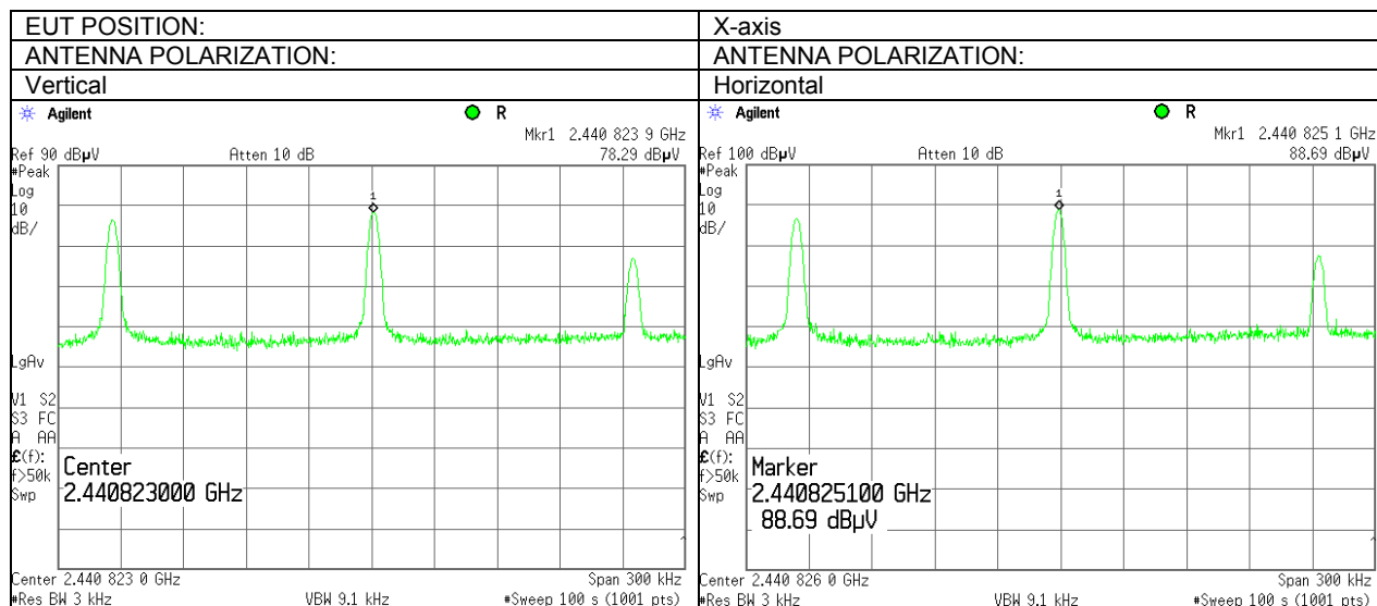
Plot 7.4.4 Peak spectral power density at mid frequency 2441 MHz zoomed at the peak
