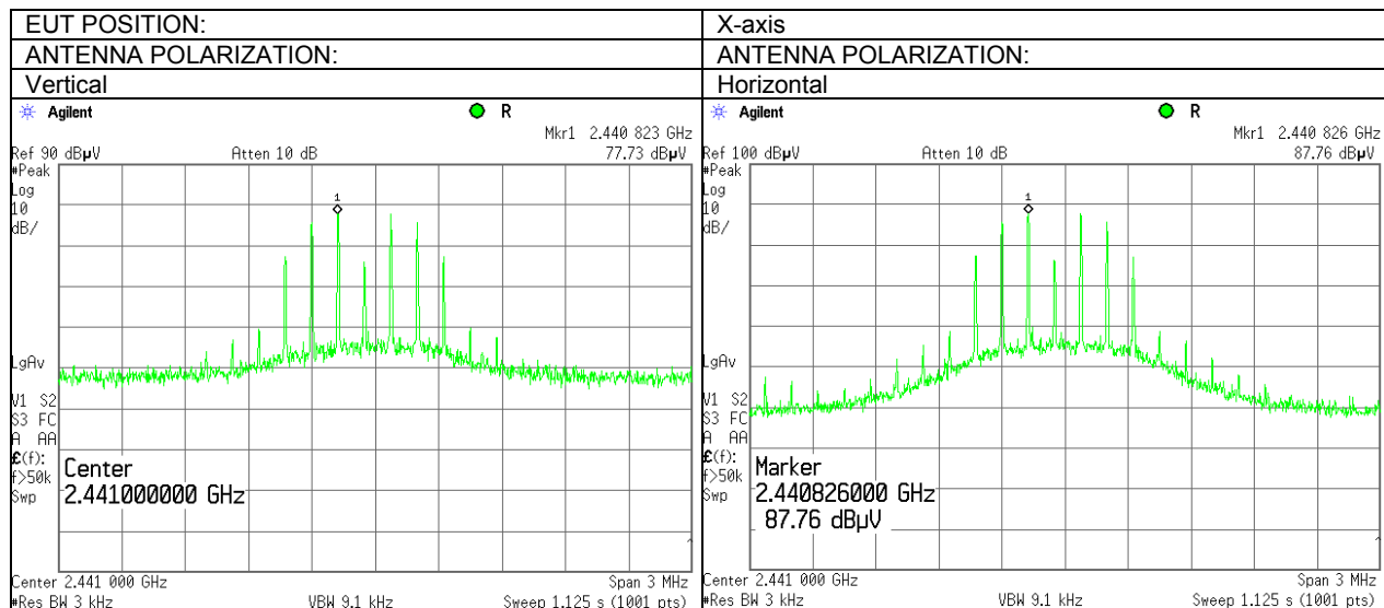
Plot 7.4.3 Peak spectral power density at mid frequency 2441 MHz within 6 dB band
