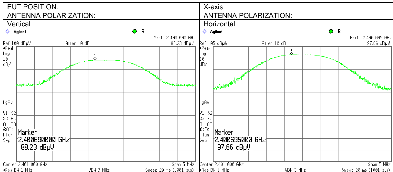
Plot 7.2.1 Field strength of carrier at low frequency and Unom
