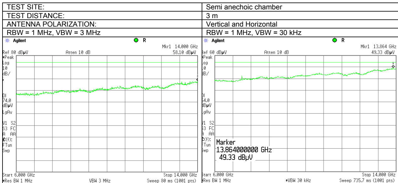
Plot 7.3.25 Radiated emission measurements from 6000 to 14000 MHz at the low carrier frequency
