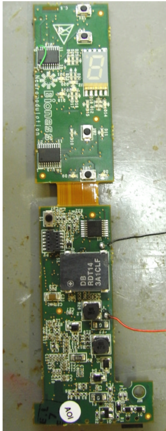
Photograph No.2 Control unit two PCBs view
