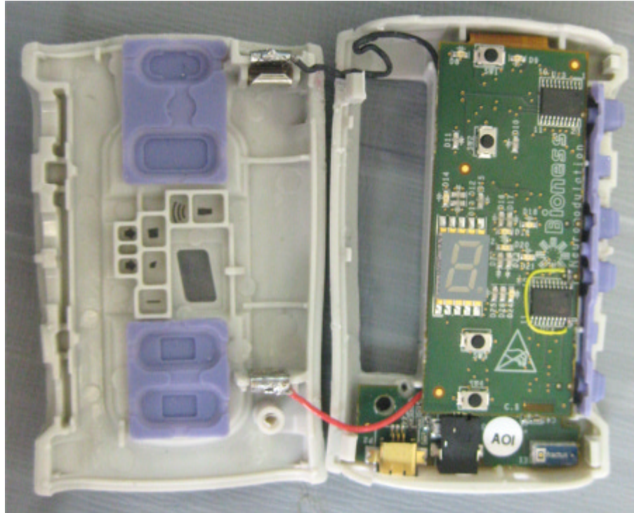
Photograph No.1 Control unit internal view
