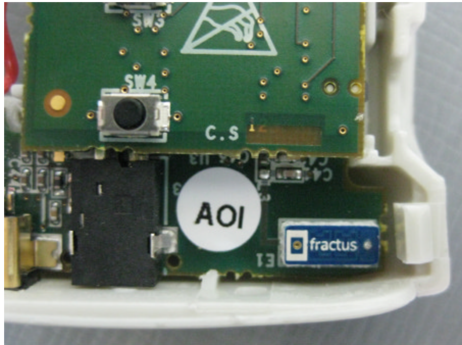
Photograph No.4 Control unit antenna close view
