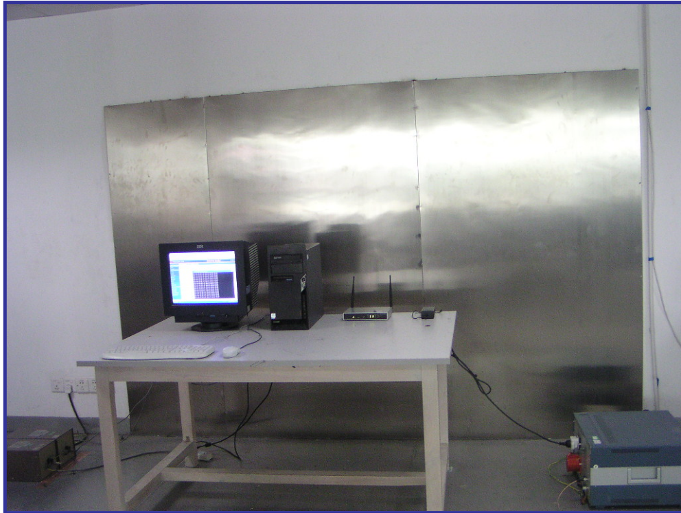
Conducted Emissions - Front View for Adapter mode
