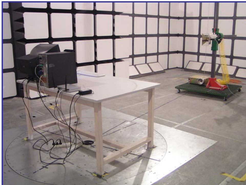
Radiated Emissions –Side View (Above 1GHz)
