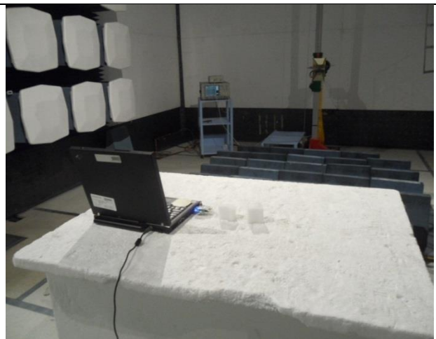
Radiated Emissions (>1GHz) – Rear View (Int. Antennas)
