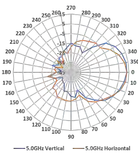
5.0GHz Horizontal Polarization
