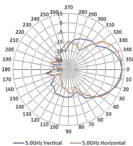
5.0GHz Vertical Polarization
