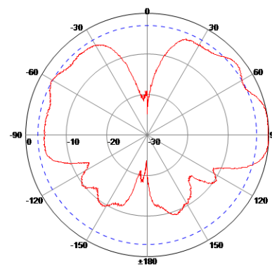
E Plane
