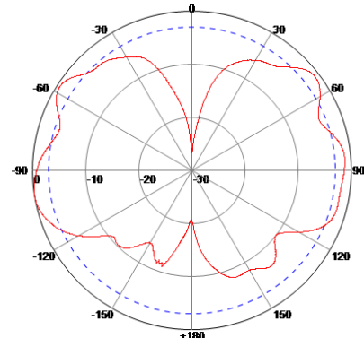
E Plane
