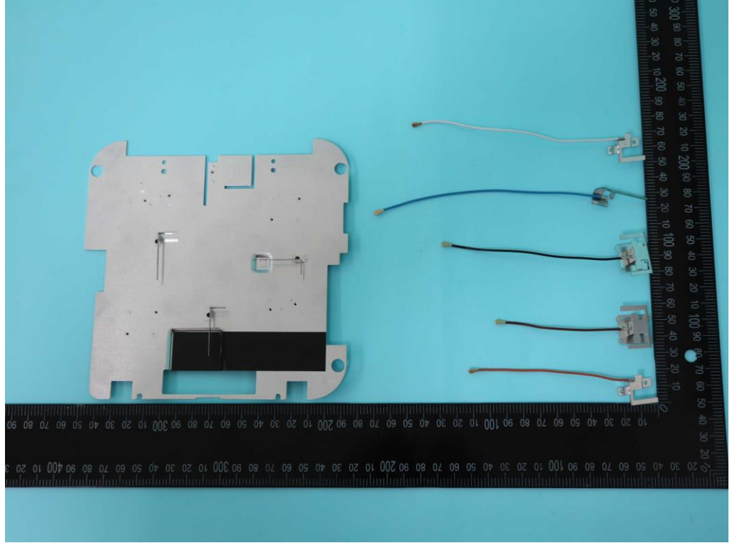
Antenna 1
