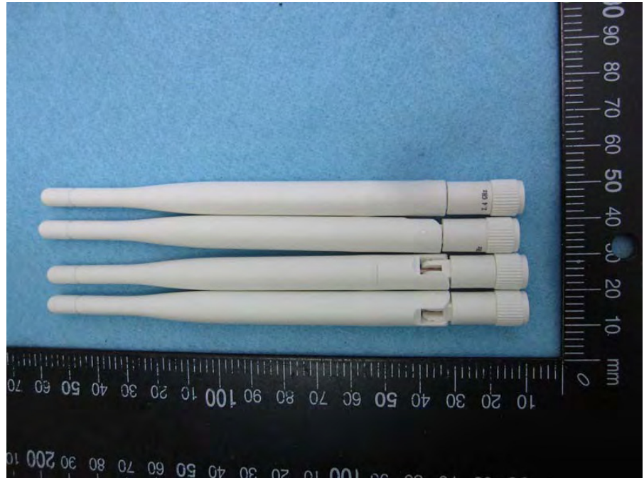
Dipole Antenna-2.4GHz (for external antenna EUT)
