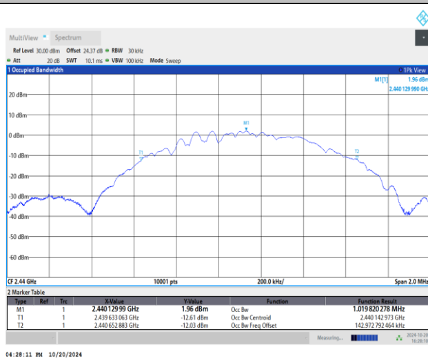
99% Occupied Bandwidth Plot on Channel 19
