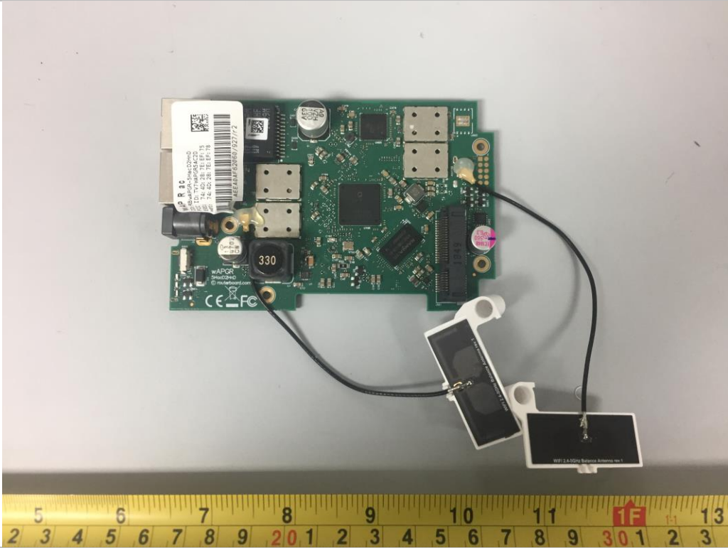
Main PCBA -Top
