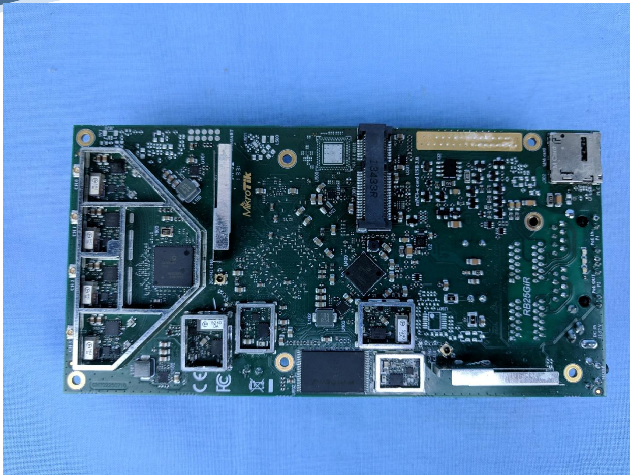
Main Board Top View No Shields
