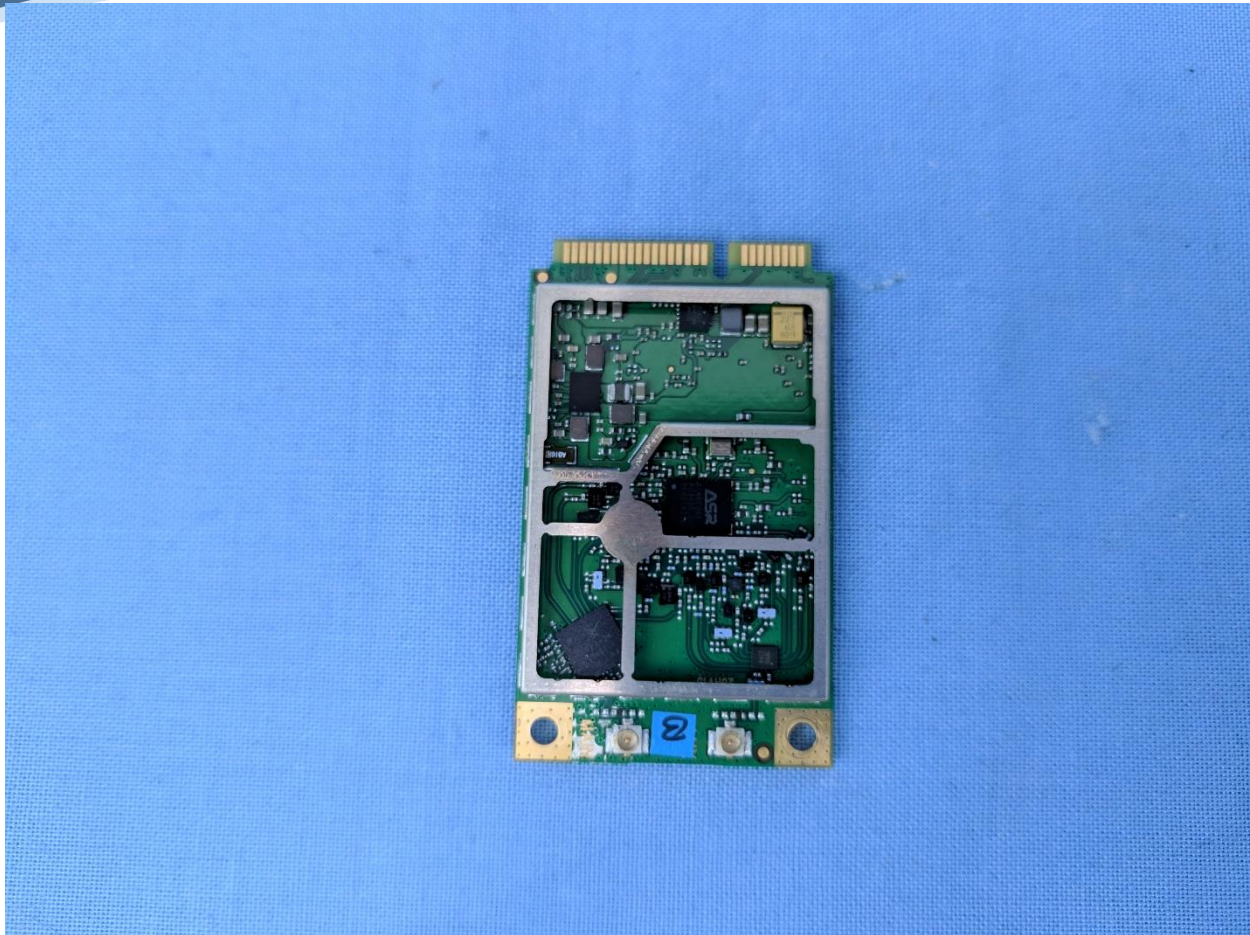
R11e-LTE6 Front No Shields
