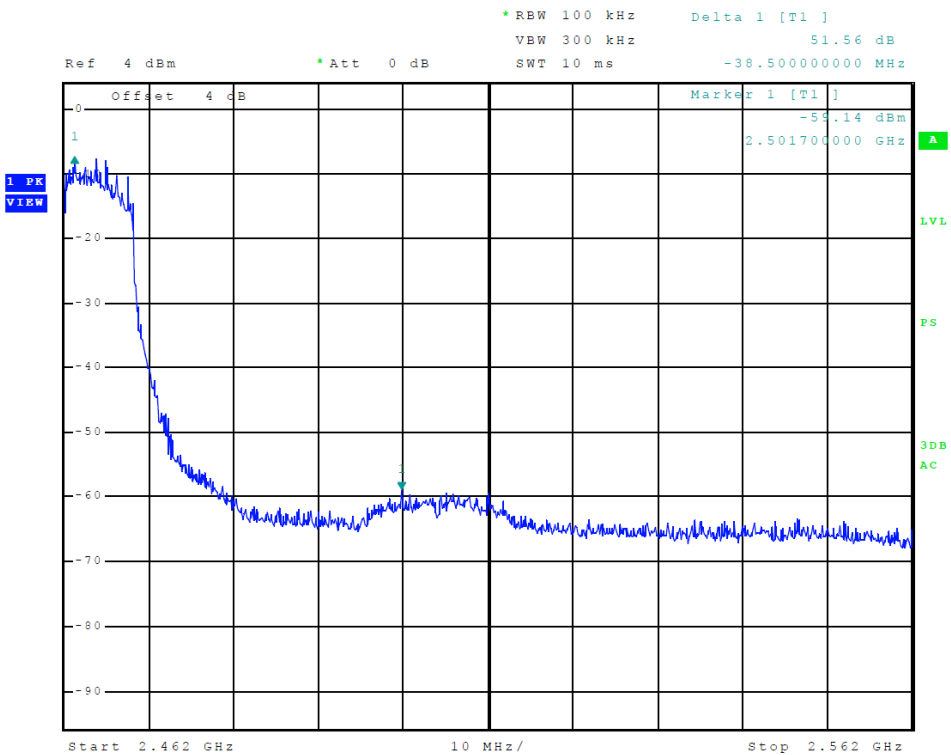
Figure 24 Plot of Transmitter High Band Edge (802.11n (20), Chain 1)
