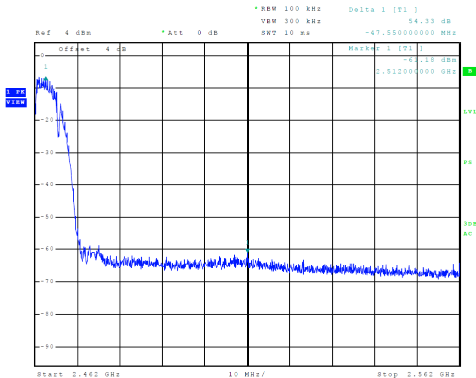
Figure 20 Plot of Transmitter High Band Edge (802.11b, Chain 1)
