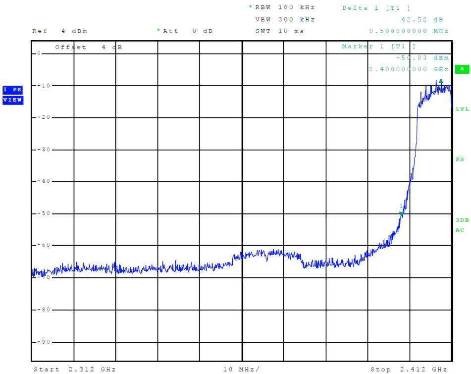
Figure 16 Plot of Transmitter Low Band Edge (802.11n (20), Chain 1)
