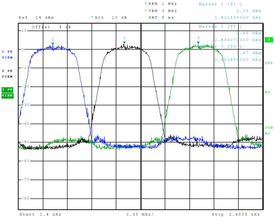
Figure 8 Plot of Transmitter Emissions (Across Operational Band, 802.11n (20), Chain 1)
