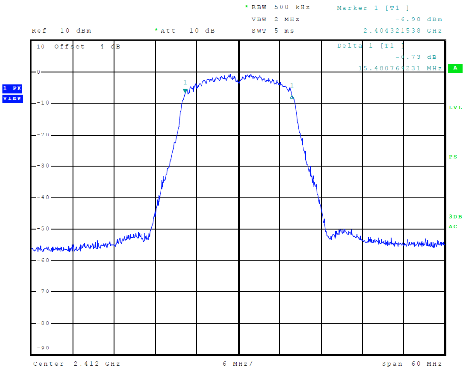
Figure 32 Plot of Transmitter 6-dB Occupied Band Width (802.11n (20), Chain 1)
