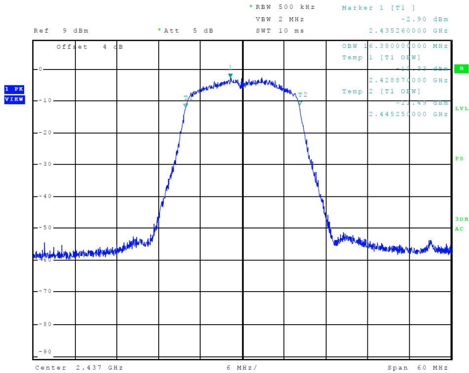
Figure 39 Plot of Transmitter 99% Occupied Band Width (802.11n (20), Chain 0)
