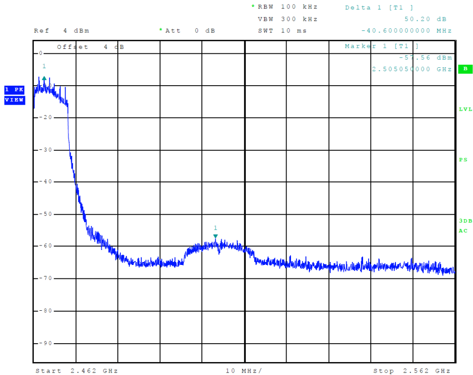
Figure 23 Plot of Transmitter High Band Edge (802.11n (20), Chain 0)
