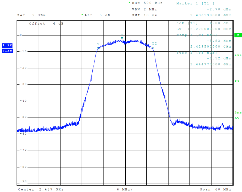
Figure 31 Plot of Transmitter 6-dB Occupied Band Width (802.11n (20), Chain 0)
