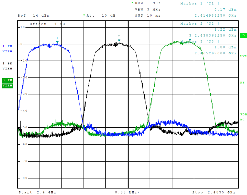
Figure 7 Plot of Transmitter Emissions (Across Operational Band, 802.11n (20), Chain 0)
