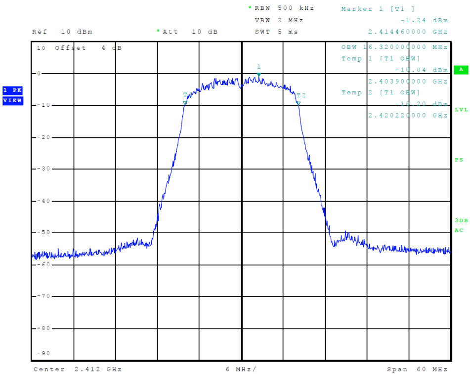
Figure 40 Plot of Transmitter 99% Occupied Band Width (802.11n (20), Chain 1)
