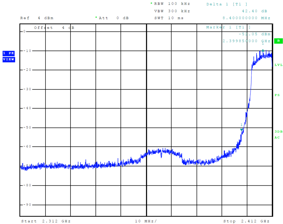
Figure 15 Plot of Transmitter Low Band Edge (802.11n (20), Chain 0)
