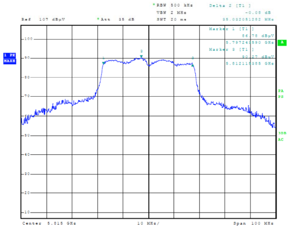
Figure Nineteen Plot of 6dB Band width (40 MHz Mode, 5815 MHz)
