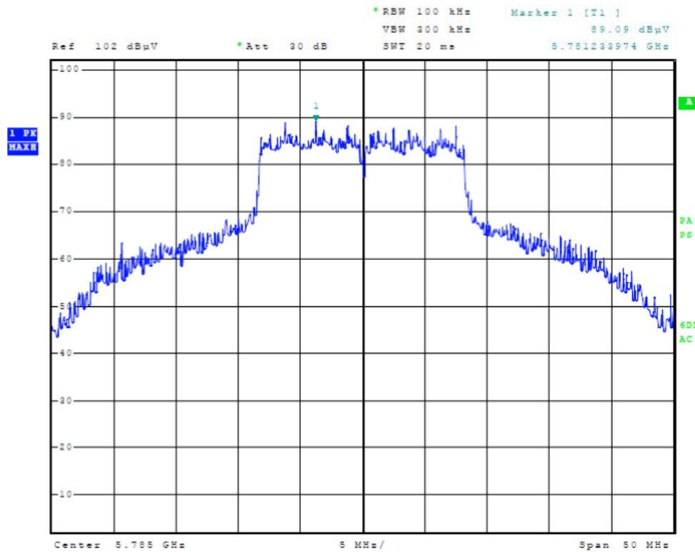
Figure Twenty-one Plot of Power Spectral Density (20 MHz Mode, 5785 MHz)
