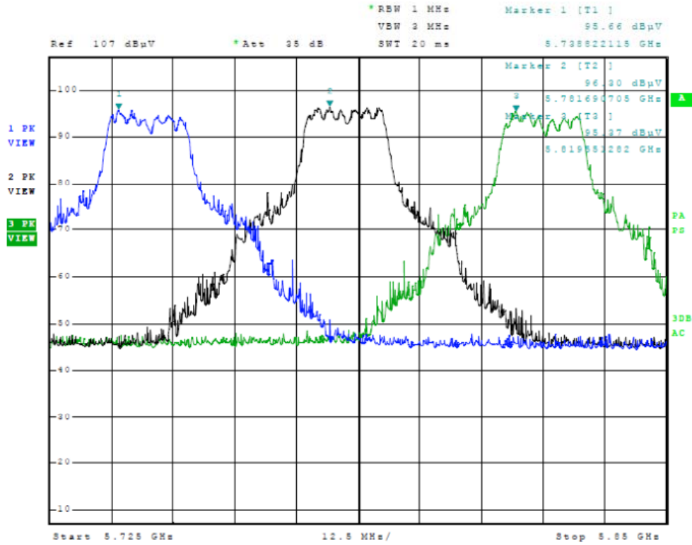
Figure Twelve Plot of Transmitter Emissions (Across Operational Band, 20MHz Mode)
