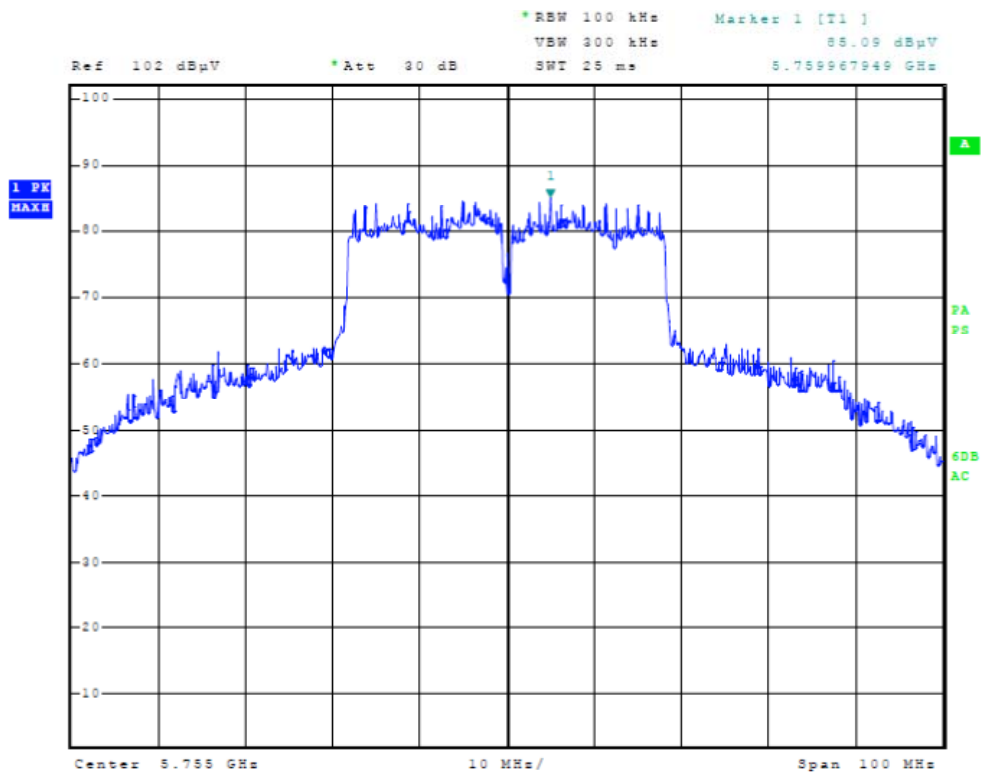
Figure Twenty-three Plot of Power Spectral Density (40 MHz Mode, 5755 MHz)
