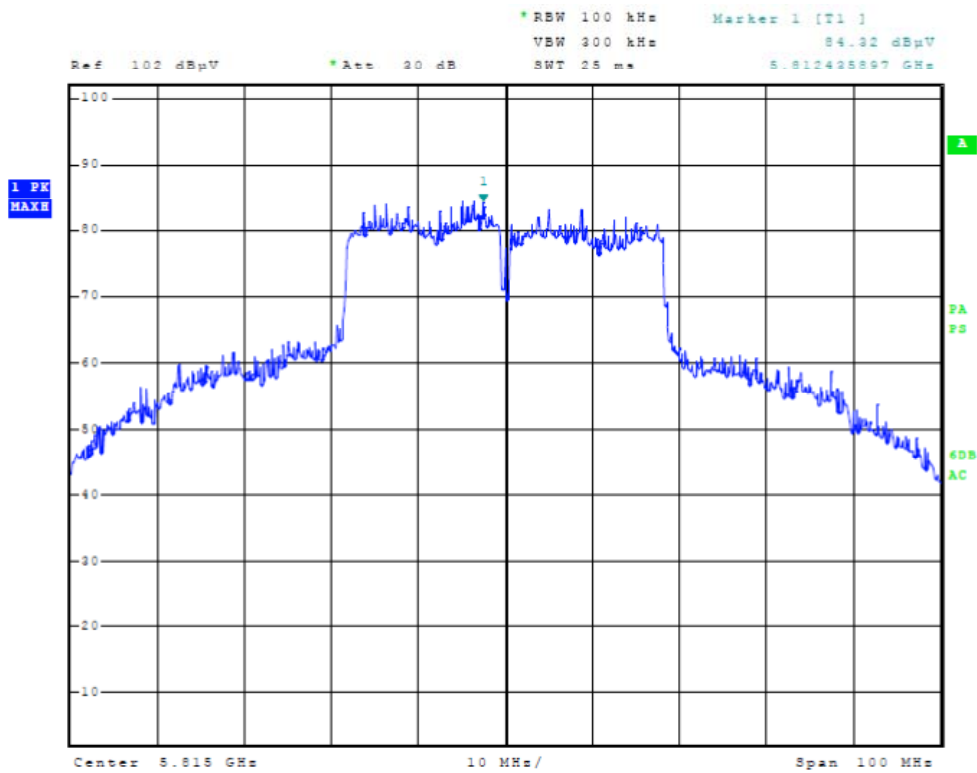
Figure Twenty-five Plot of Power Spectral Density (40 MHz Mode, 5815 MHz)
