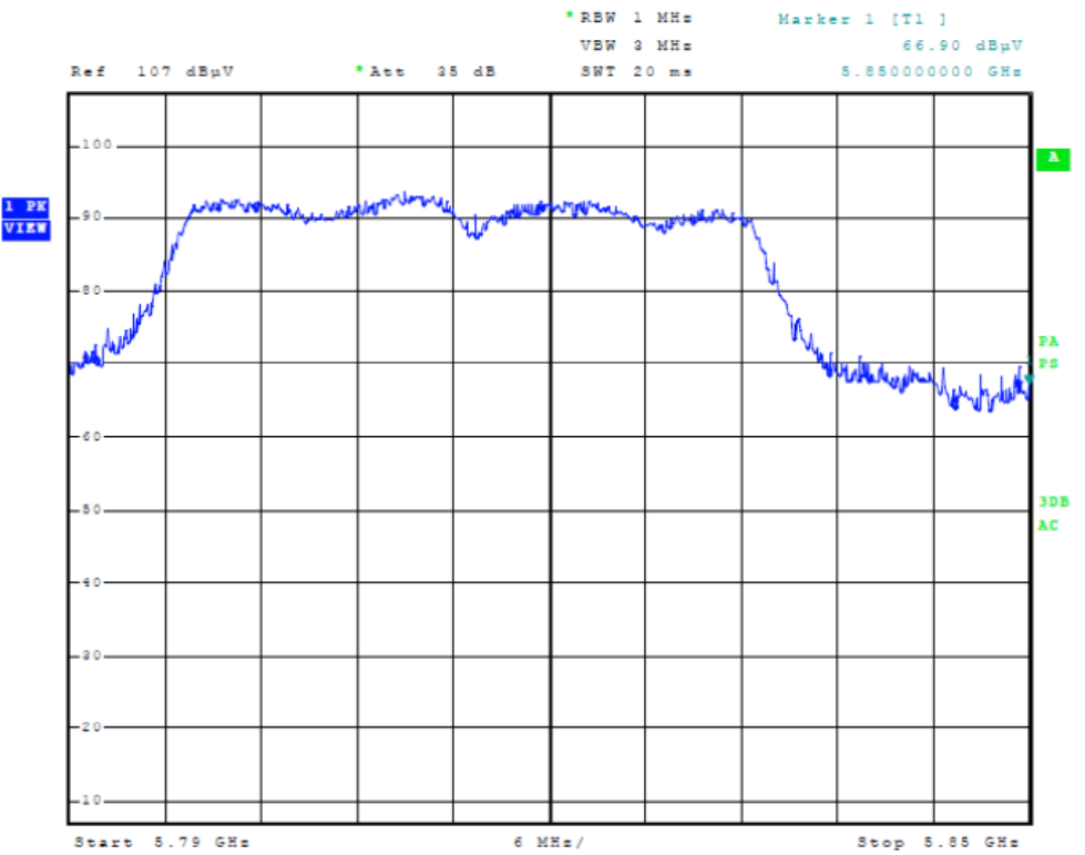
Figure Twenty-nine Plot of Upper Band Edge (40 MHz Mode)
