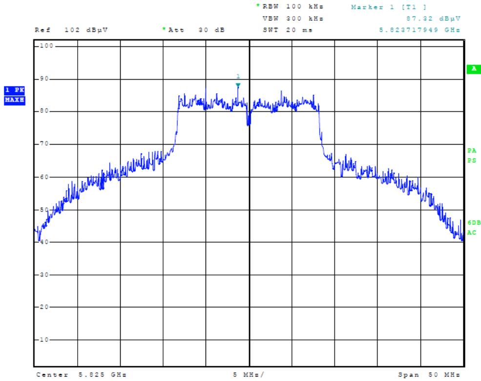
Figure Twenty-two Plot of Power Spectral Density (20 MHz Mode, 5825 MHz)
