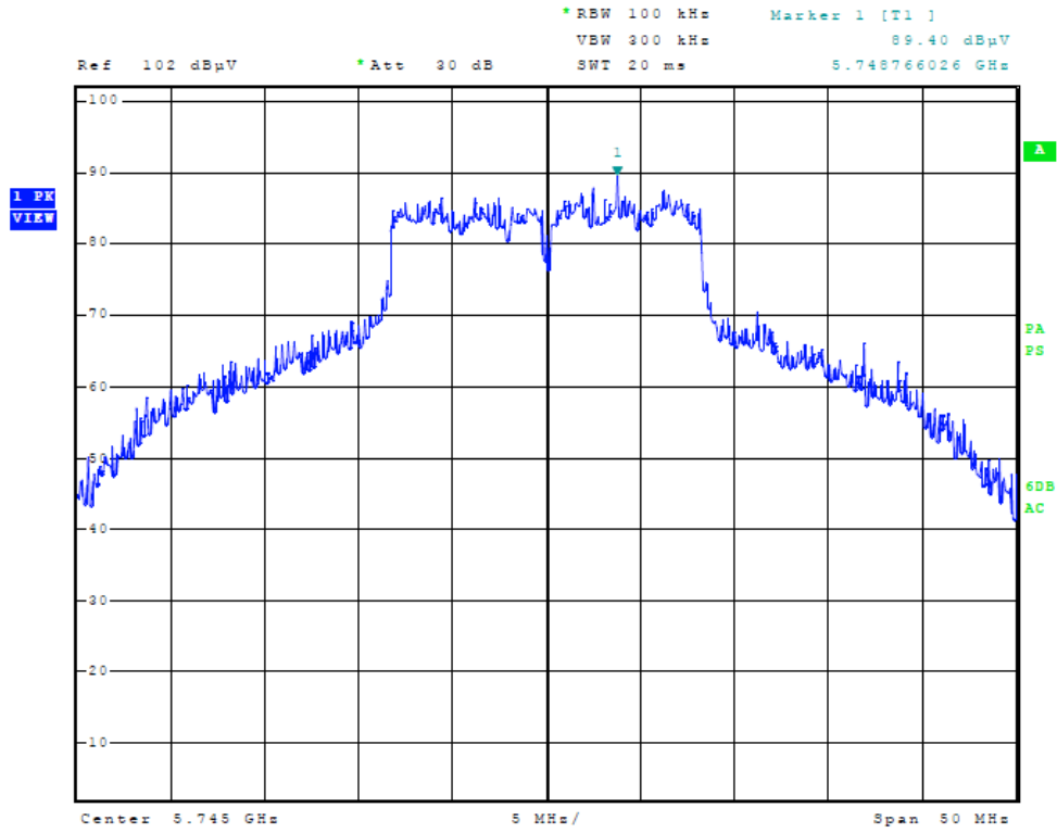
Figure Twenty Plot of Power Spectral Density (20 MHz Mode, 5745 MHz)
