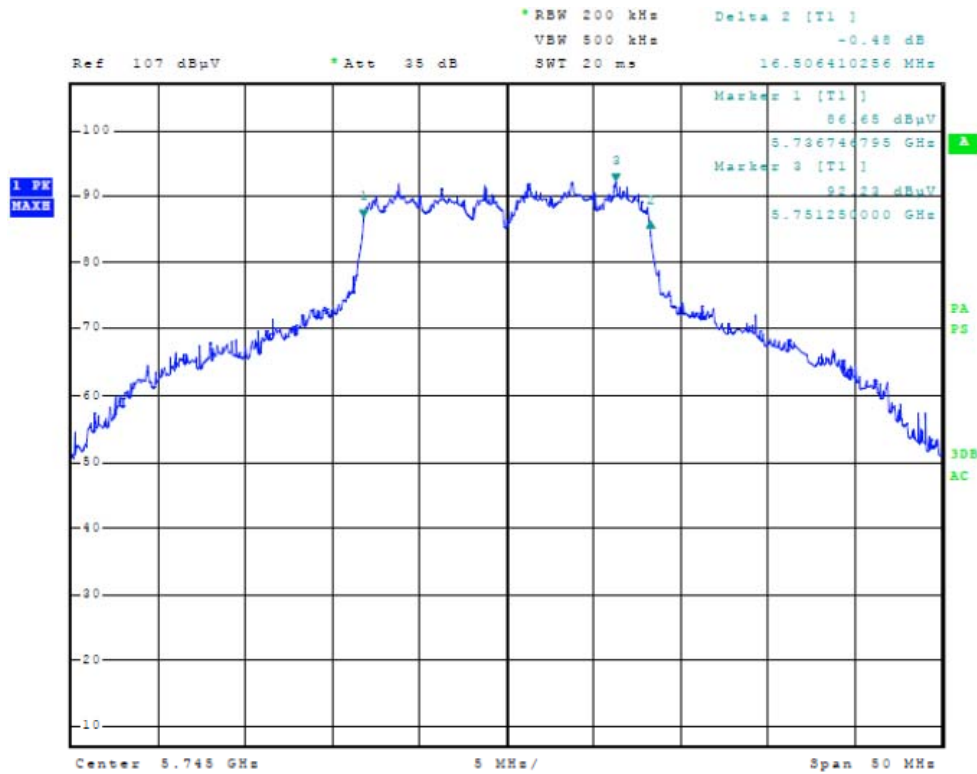
Figure Fourteen Plot of 6dB Band width (20 MHz Mode, 5745 MHz)
