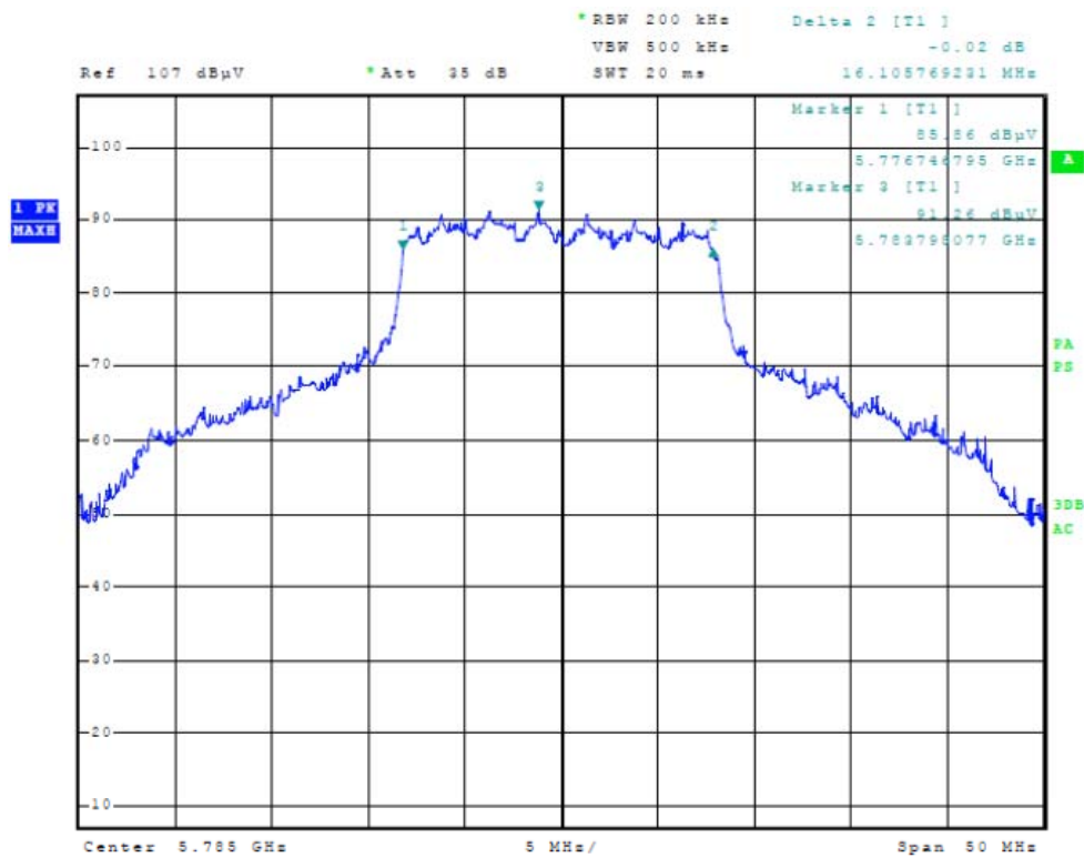
Figure Fifteen Plot of 6dB Band width (20 MHz Mode, 5785 MHz)
