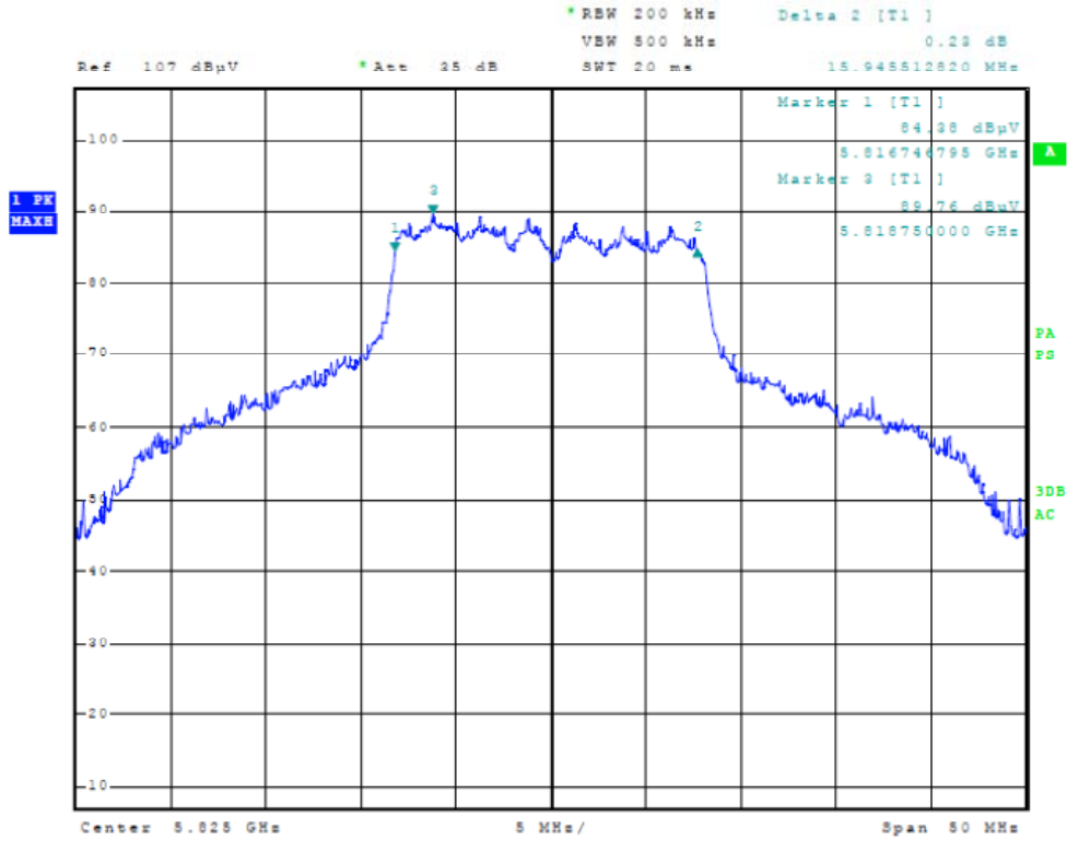
Figure Sixteen Plot of 6dB Band width (20 MHz Mode, 5825 MHz)
