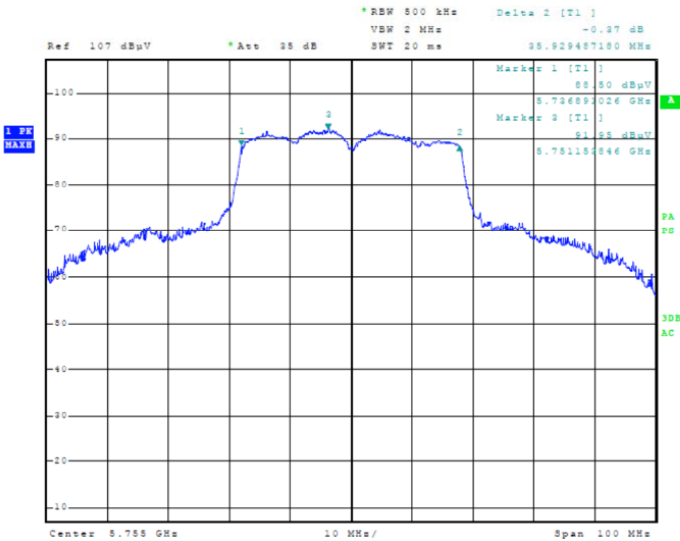
Figure Seventeen Plot of 6dB Band width (40 MHz Mode, 5755 MHz)
