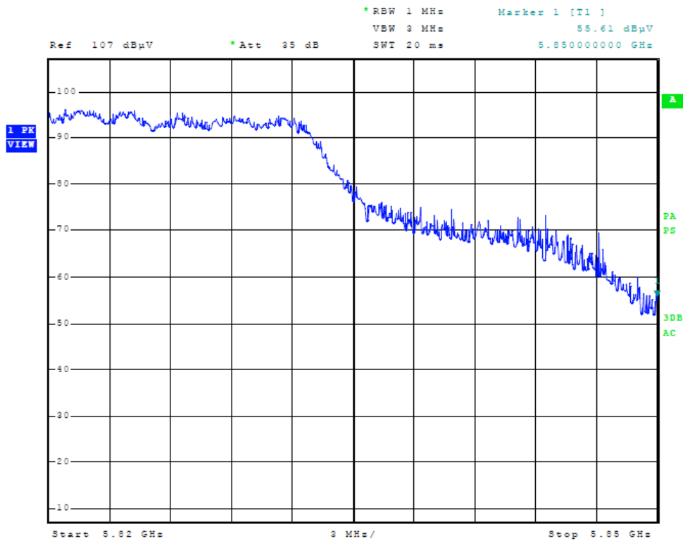
Figure Twenty-seven Plot of Upper Band Edge (20 MHz Mode)
