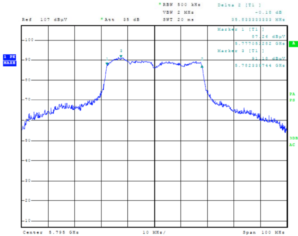
Figure Eighteen Plot of 6dB Band width (40 MHz Mode, 5795 MHz)
