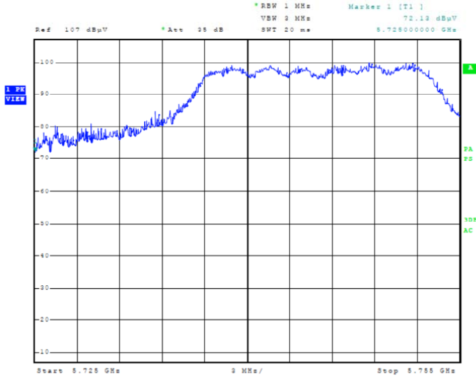
Figure Twenty-six Plot of Lower Band Edge (20 MHz Mode)
