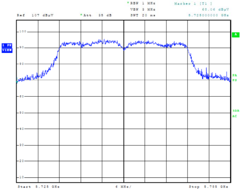
Figure Twenty-eight Plot of Lower Band Edge (40 MHz Mode)
