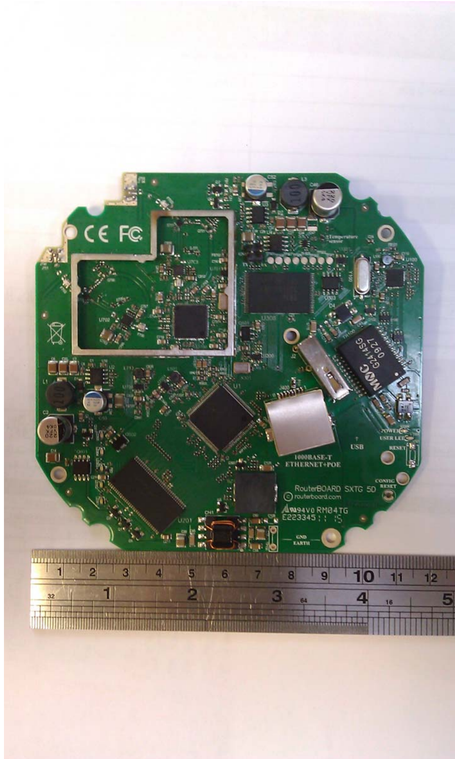
Internal photographs of equipment under test PCB without shield
