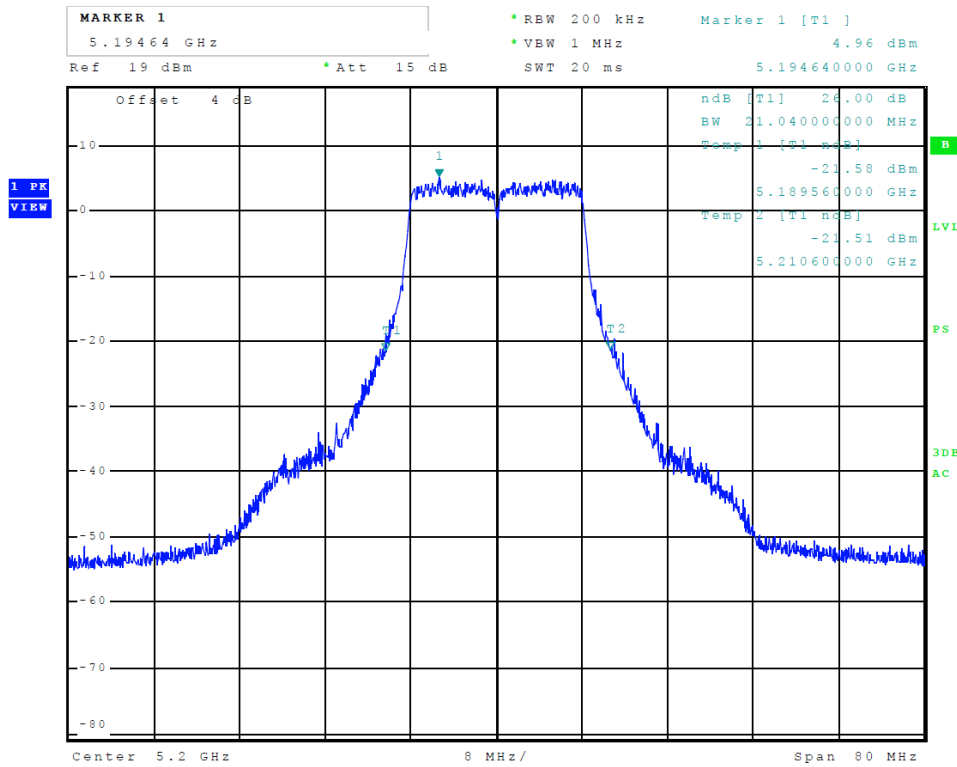
Figure 27 Plot of Transmitter Emissions (Chain 0, 5150-5250 MHz Band, 802.11a, 26 dB OBW)
