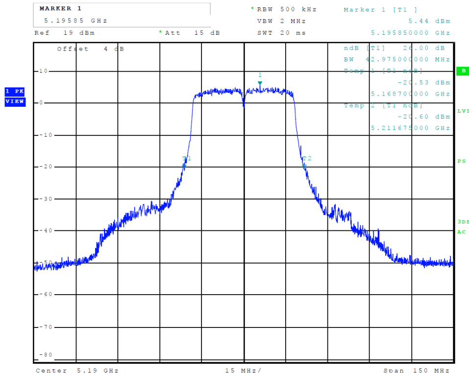
Figure 30 Plot of Transmitter Emissions (Chain 1, 5150-5250 MHz Band, 802.11n40, 26 dB OBW)
