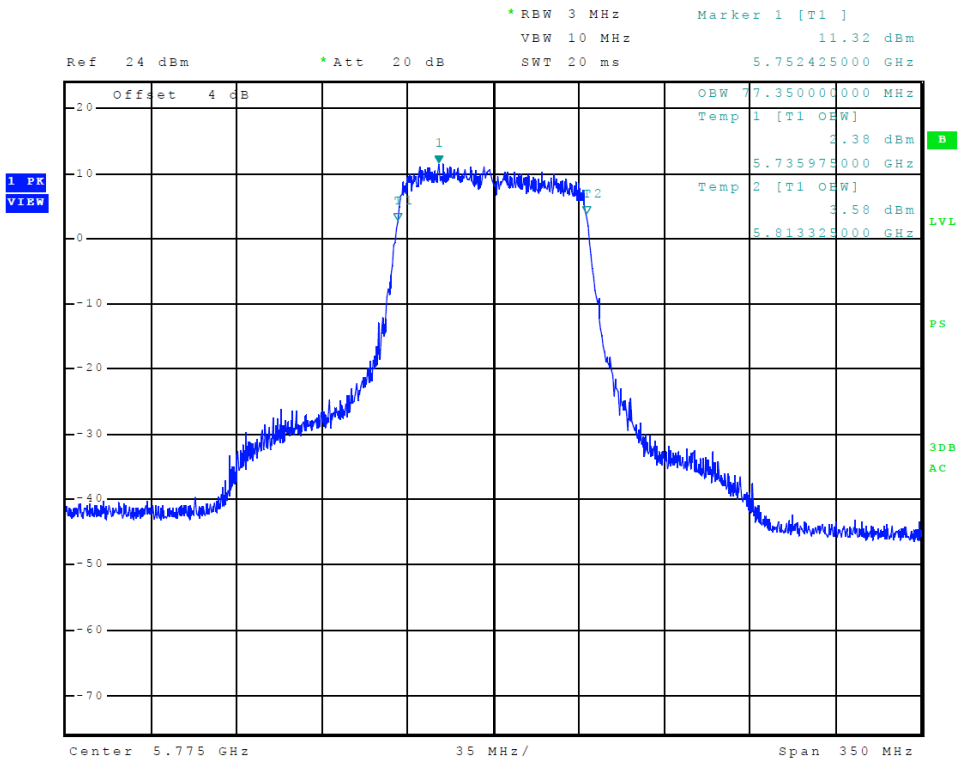
Figure 56 Plot of Transmitter Emissions (Chain 1, 5725-5850 MHz Band, 802.11ac80, 99% OBW)
