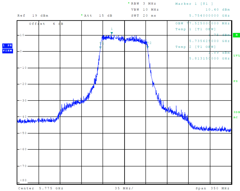
Figure 55 Plot of Transmitter Emissions (Chain 0, 5725-5850 MHz Band, 802.11ac80, 99% OBW)
