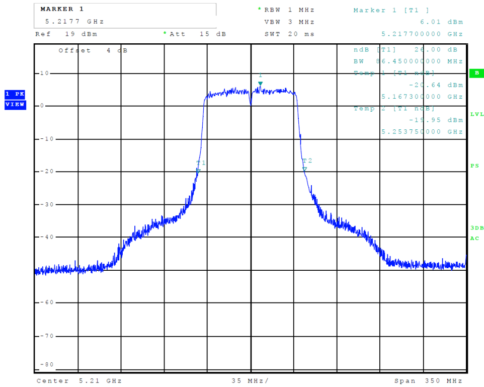
Figure 31 Plot of Transmitter Emissions (Chain 0, 5150-5250 MHz Band, 802.11ac, 26 dB OBW)
