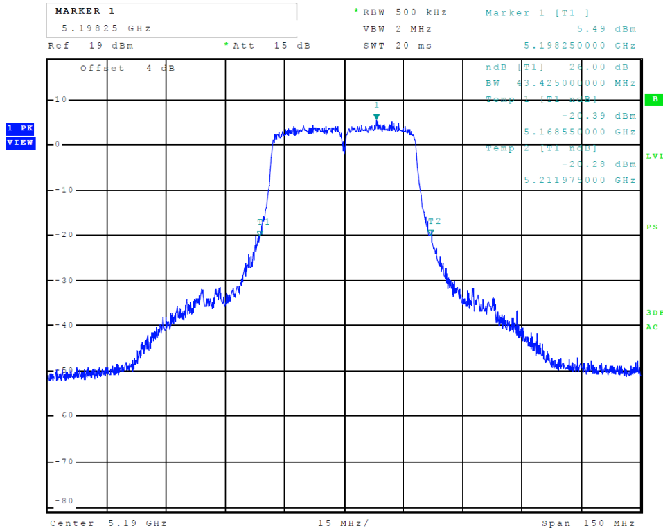
Figure 29 Plot of Transmitter Emissions (Chain 0, 5150-5250 MHz Band, 802.11n40, 26 dB OBW)
