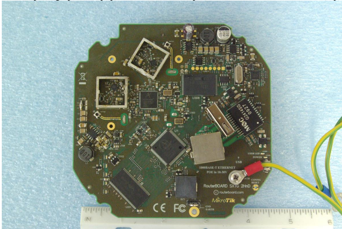
Internal photographs of equipment under test component side with shields removed (top)
