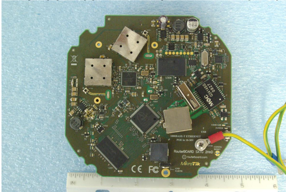
Internal photographs of equipment under test component side with shields in place (top)
