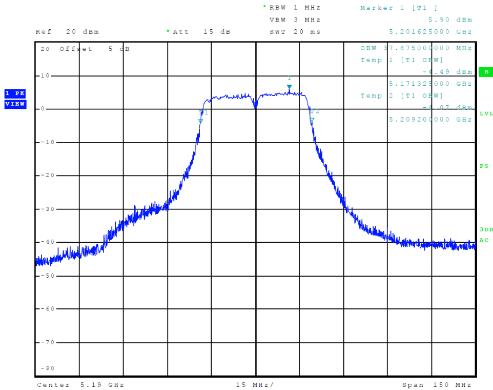
Figure 19 Plot of Transmitter Emissions (Chain 0, 5150-5250 MHz Band, 802.11n40, 99% OBW)
