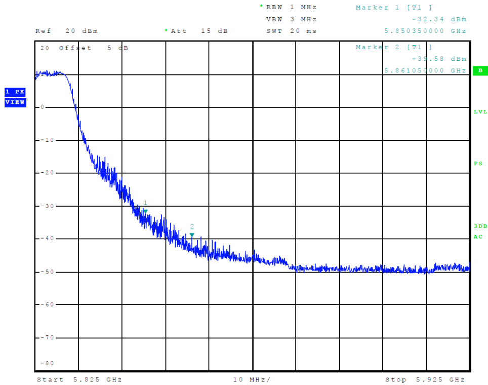
Figure 31 Plot of Transmitter High Band Edge (Chain 0, 5725-5850 MHz Band, 802.11a)
