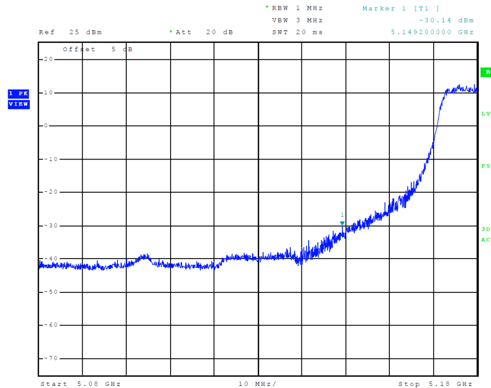
Figure 8 Plot of Transmitter Low Band Edge (Chain 1, 5150-5250 MHz Band, 802.11a)
