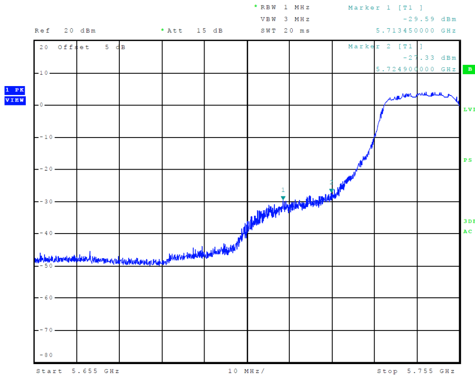
Figure 29 Plot of Transmitter Low Band Edge (Chain 0, 5725-5850 MHz Band, 802.11n40)
