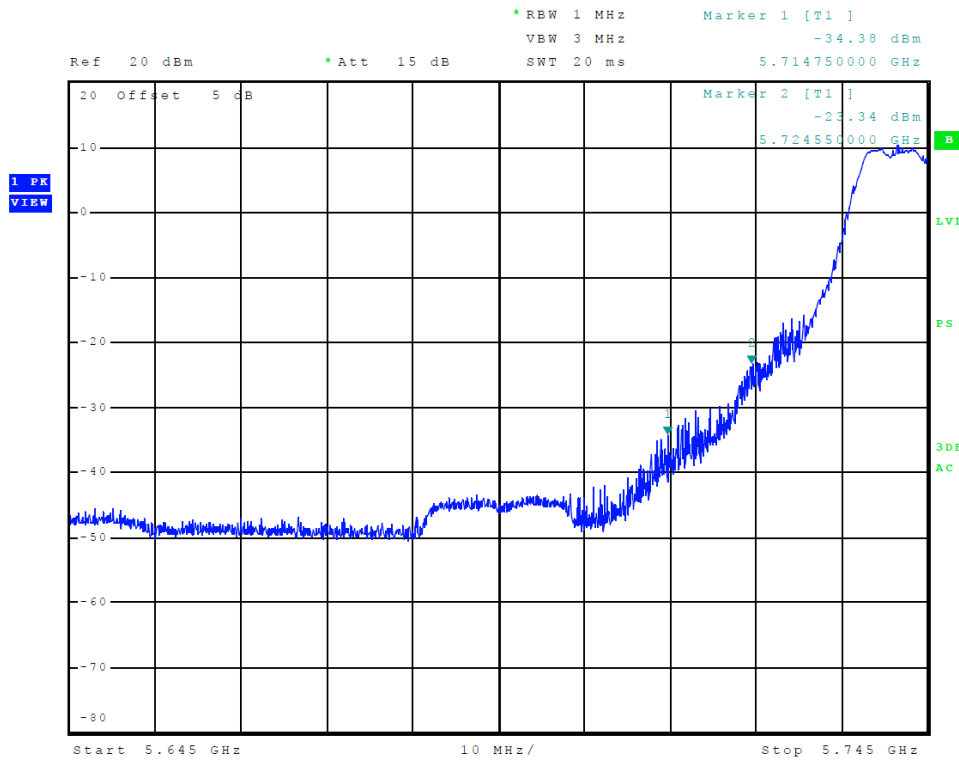
Figure 27 Plot of Transmitter Low Band Edge (Chain 0, 5725-5850 MHz Band, 802.11a)
