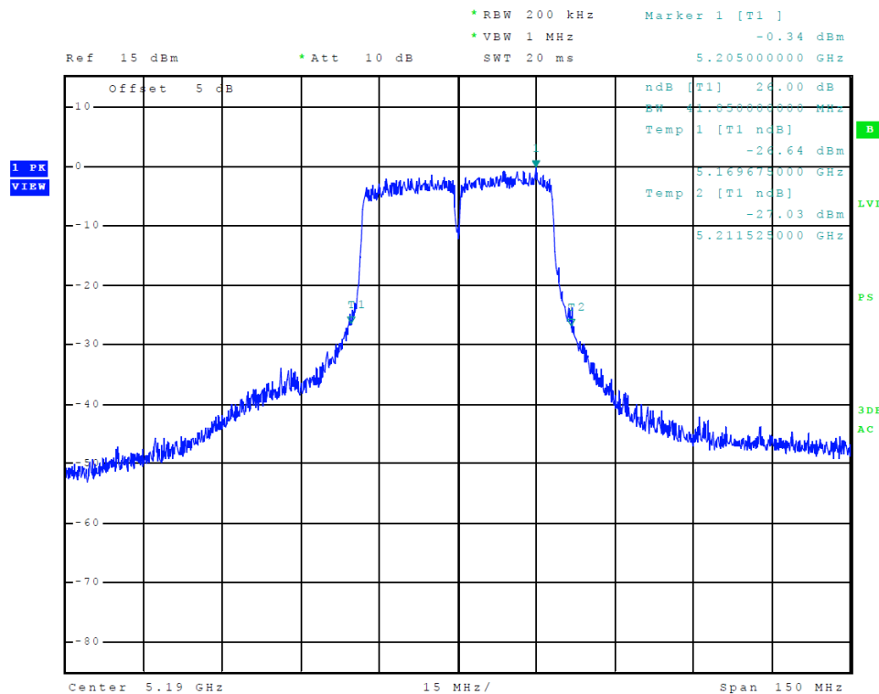
Figure 22 Plot of Transmitter Emissions (Chain 1, 5150-5250 MHz Band, 802.11n40, 26 dB OBW)
