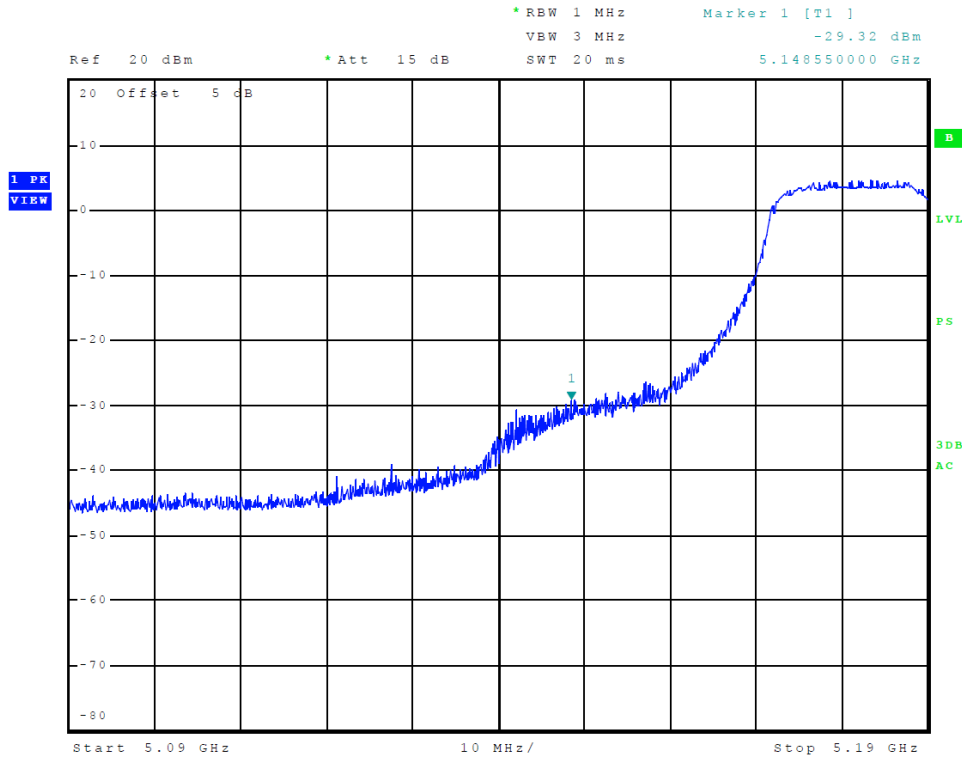
Figure 9 Plot of Transmitter Low Band Edge (Chain 0, 5150-5250 MHz Band, 802.11n40)
