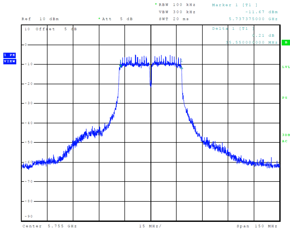
Figure 41 Plot of Transmitter Emissions (Chain 0, 5725-5850 MHz Band, 802.11n40, 6-dB OBW)
