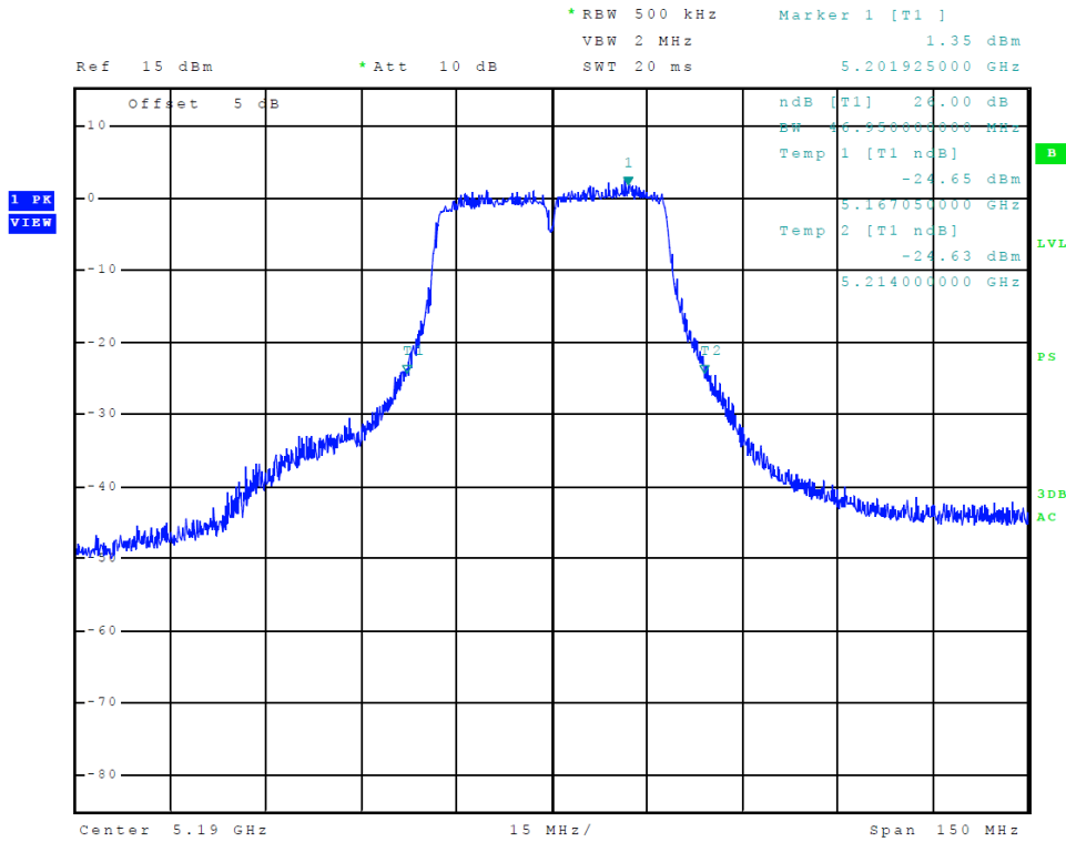
Figure 21 Plot of Transmitter Emissions (Chain 0, 5150-5250 MHz Band, 802.11n40, 26 dB OBW)
