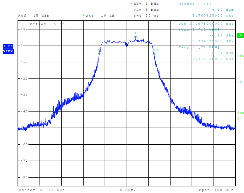
Figure 39 Plot of Transmitter Emissions (Chain 0, 5725-5850 MHz Band, 802.11n40, 99% OBW)
