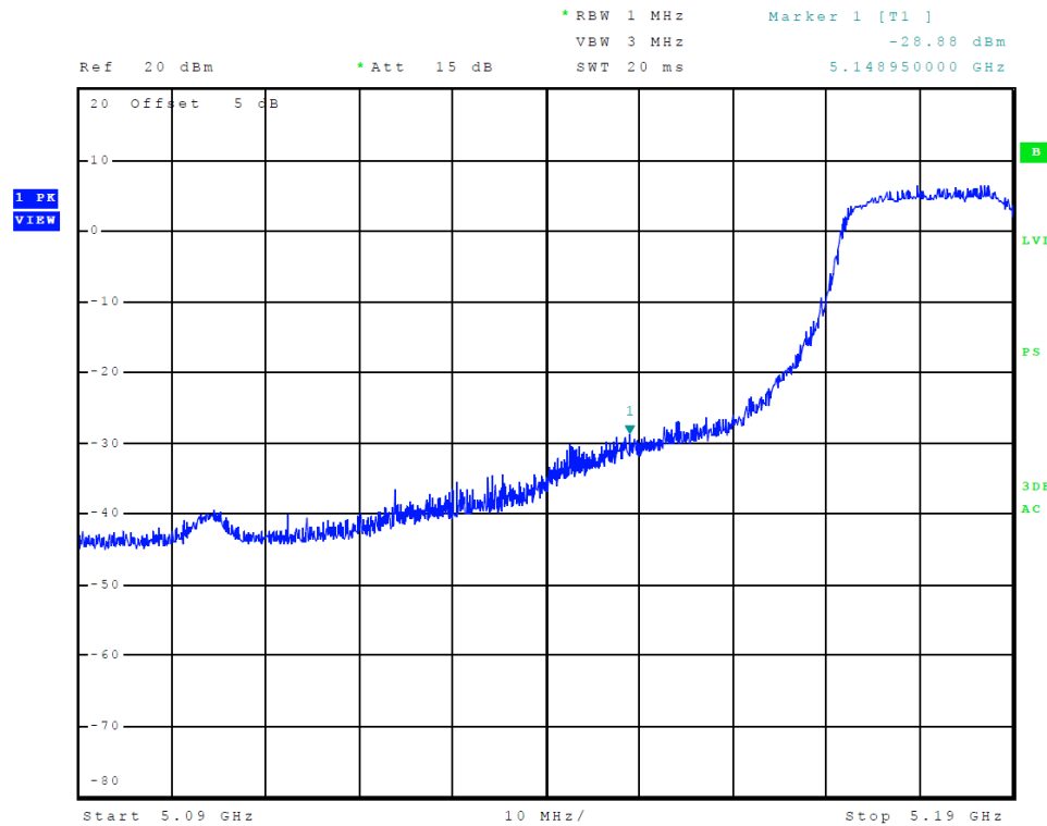
Figure 10 Plot of Transmitter Low Band Edge (Chain 1, 5150-5250 MHz Band, 802.11n40)
