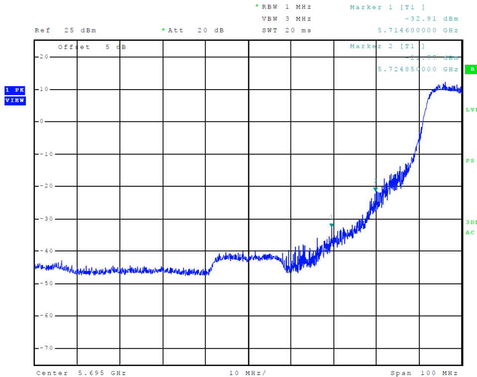
Figure 28 Plot of Transmitter Low Band Edge (Chain 1, 5725-5850 MHz Band, 802.11a)
