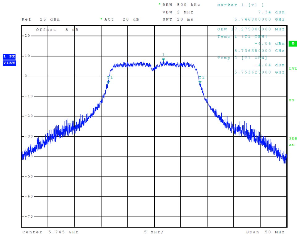
Figure 36 Plot of Transmitter Emissions (Chain 1, 5725-5850 MHz Band, 802.11a, 99% OBW)
