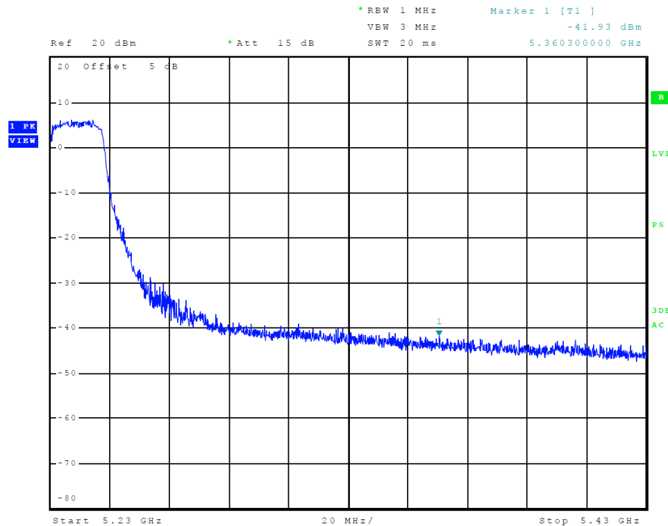
Figure 14 Plot of Transmitter High Band Edge (Chain 1, 5150-5250 MHz Band, 802.11n40)
