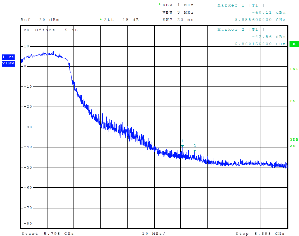
Figure 34 Plot of Transmitter High Band Edge (Chain 1, 5725-5850 MHz Band, 802.11n40)
