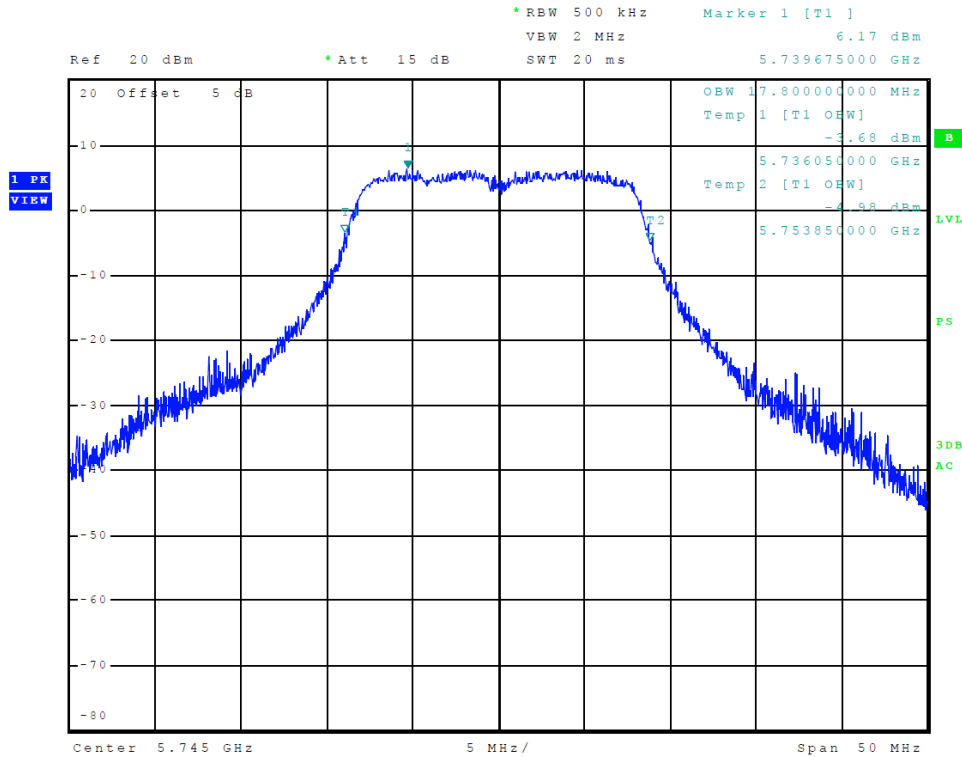
Figure 35 Plot of Transmitter Emissions (Chain 0, 5725-5850 MHz Band, 802.11a, 99% OBW)
