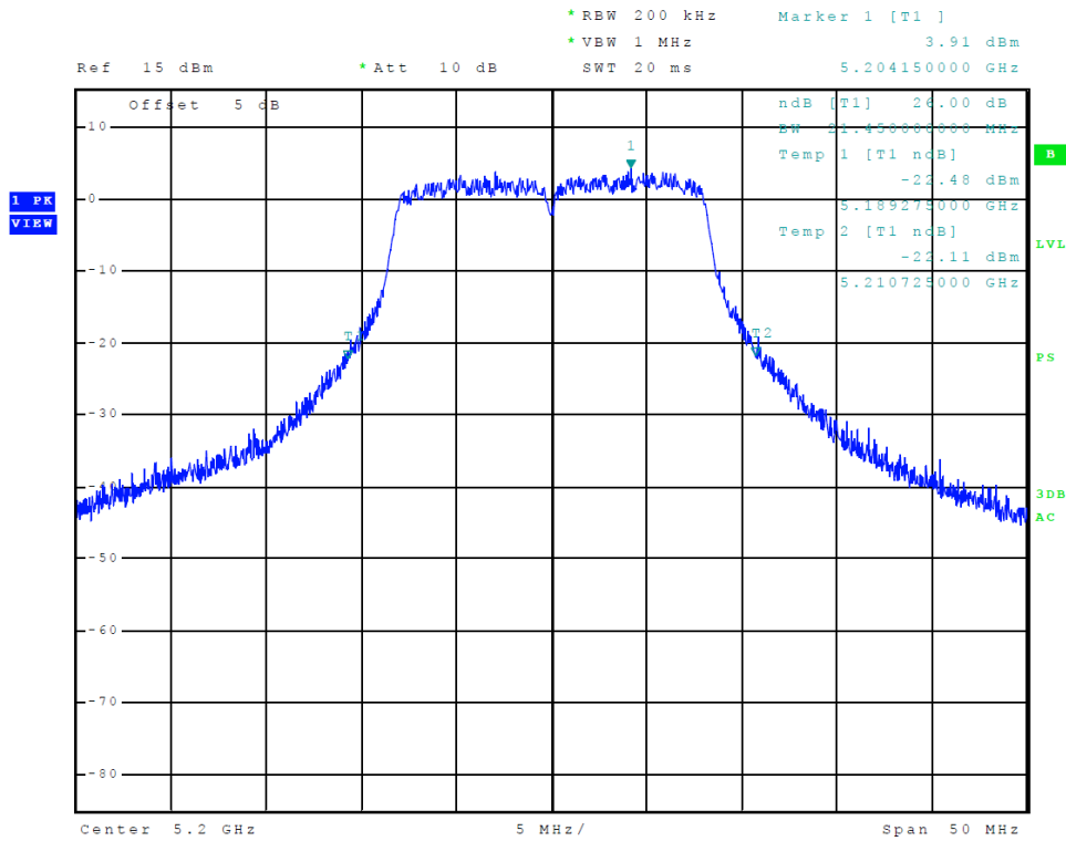
Figure 17 Plot of Transmitter Emissions (Chain 0, 5150-5250 MHz Band, 802.11a, 26 dB OBW)
