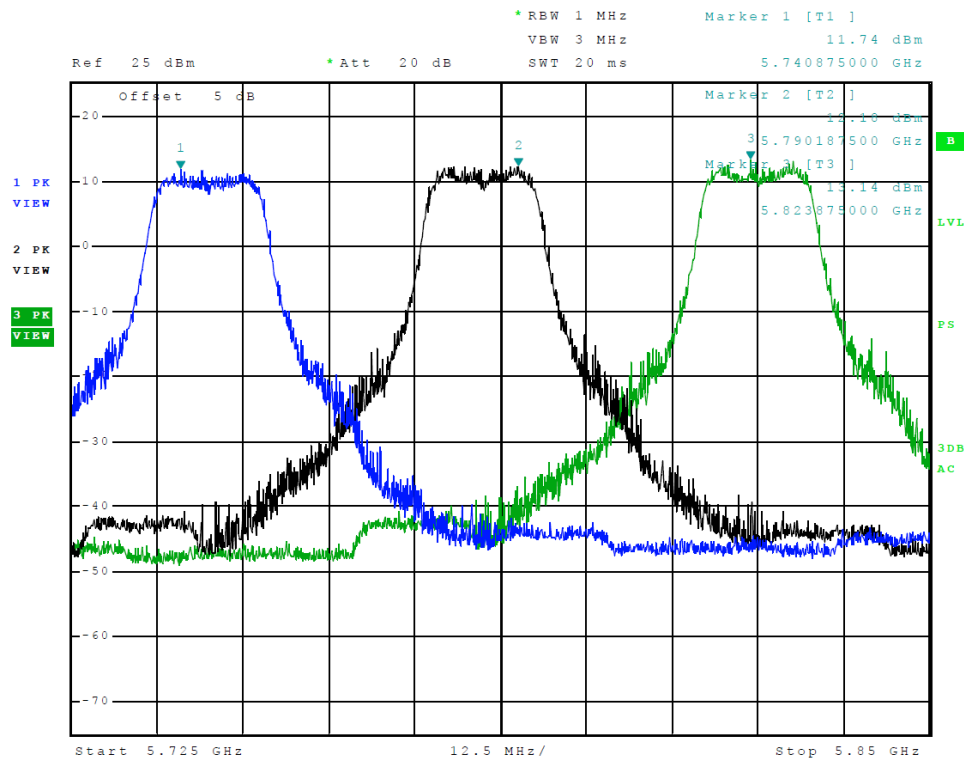
Figure 24 Plot of Transmitter Emissions (Chain 1, Across 5725-5850 MHz Band, 802.11a)
