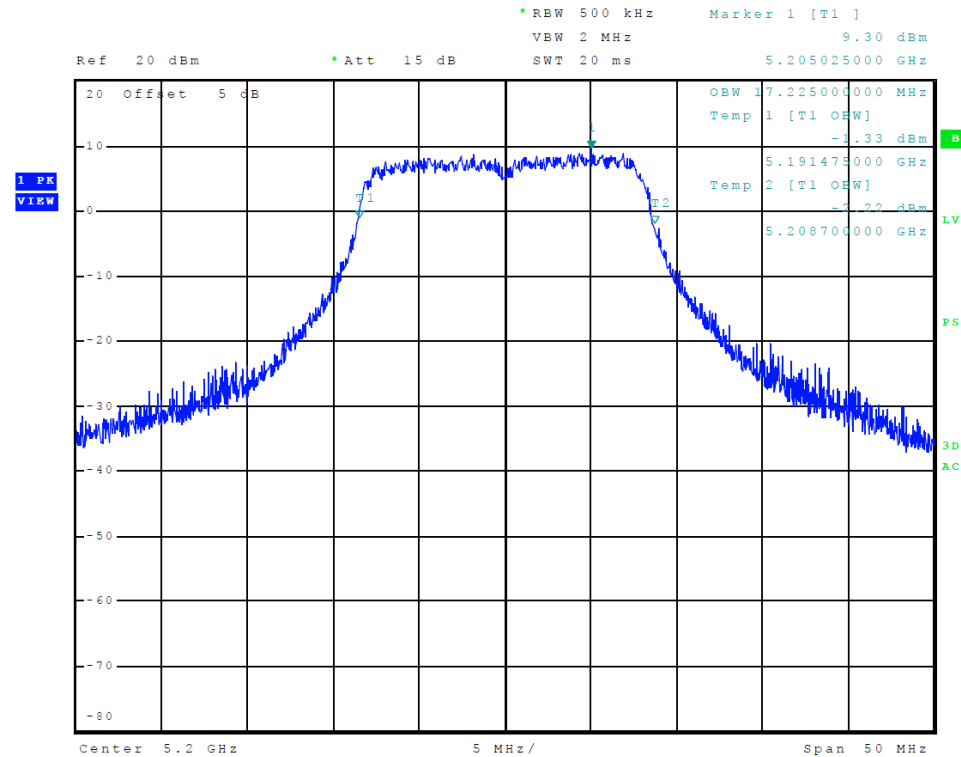
Figure 16 Plot of Transmitter Emissions (Chain 1, 5150-5250 MHz Band, 802.11a, 99% OBW)
