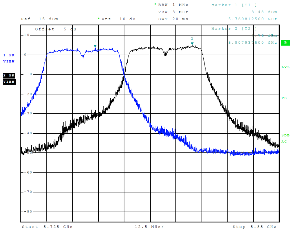
Figure 25 Plot of Transmitter Emissions (Chain 0, Across 5725-5850 MHz Band, 802.11n40)
