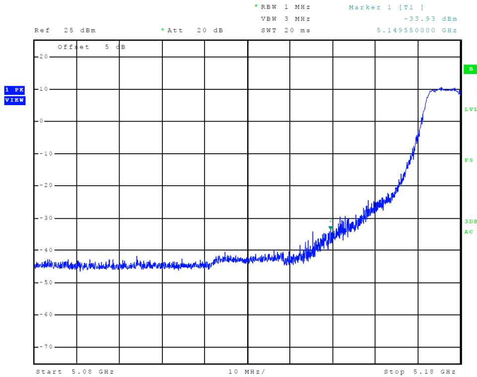
Figure 7 Plot of Transmitter Low Band Edge (Chain 0, 5150-5250 MHz Band, 802.11a)
