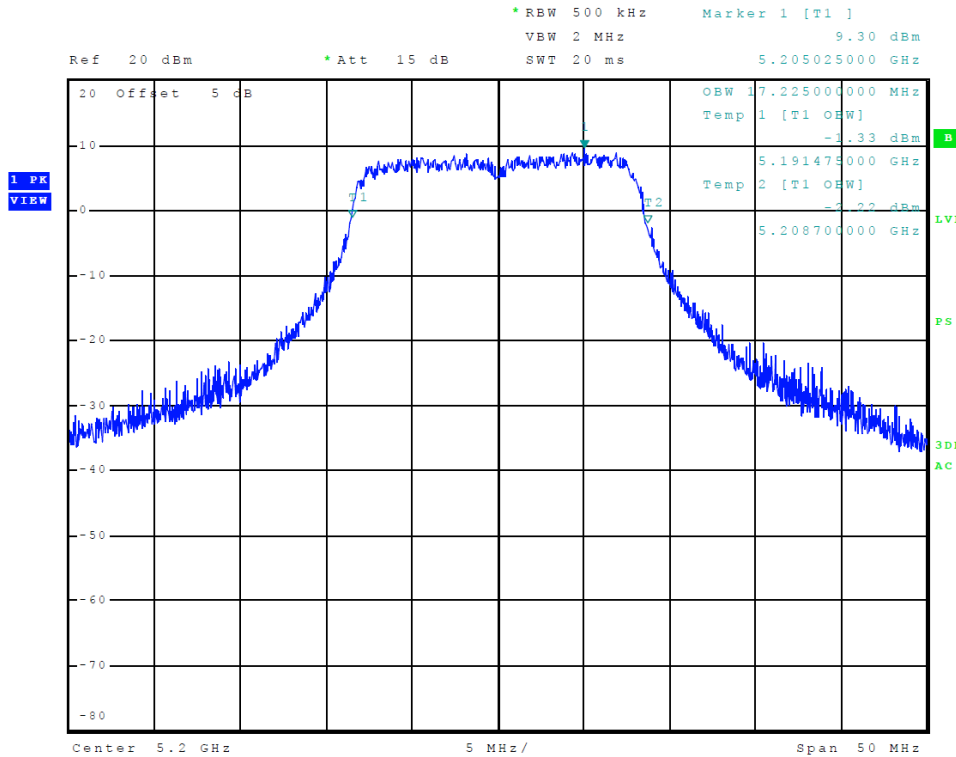
Figure 18 Plot of Transmitter Emissions (Chain 1, 5150-5250 MHz Band, 802.11a, 26 dB OBW)
