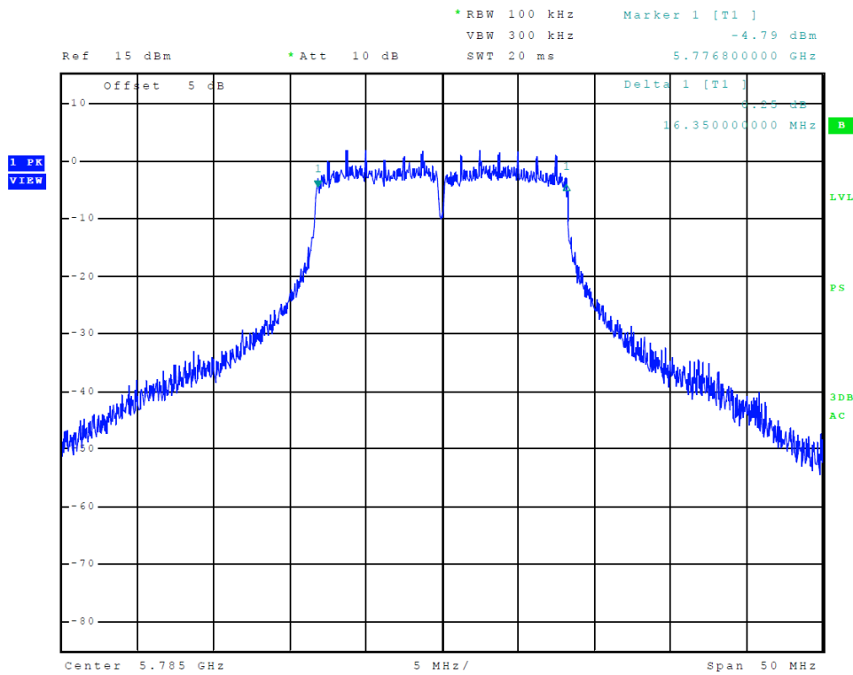
Figure 37 Plot of Transmitter Emissions (Chain 0, 5725-5850 MHz Band, 802.11a, 6-dB OBW)
