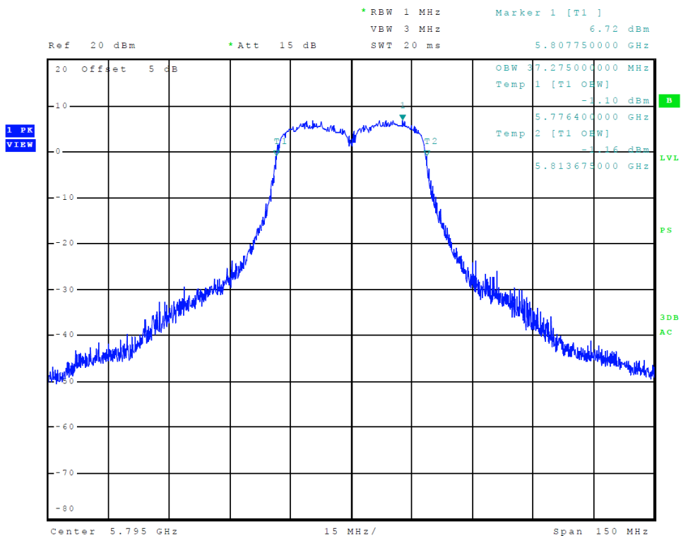
Figure 40 Plot of Transmitter Emissions (Chain 1, 5725-5850 MHz Band, 802.11n40, 99% OBW)
