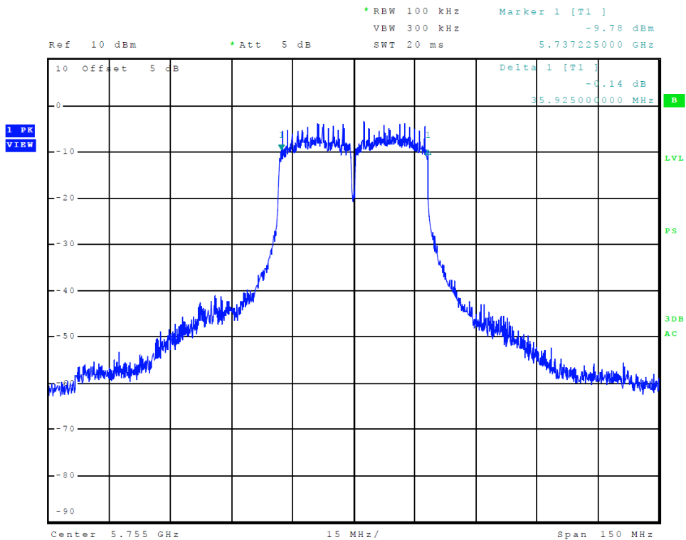
Figure 42 Plot of Transmitter Emissions (Chain 1, 5725-5850 MHz Band, 802.11n40, 6-dB OBW)
