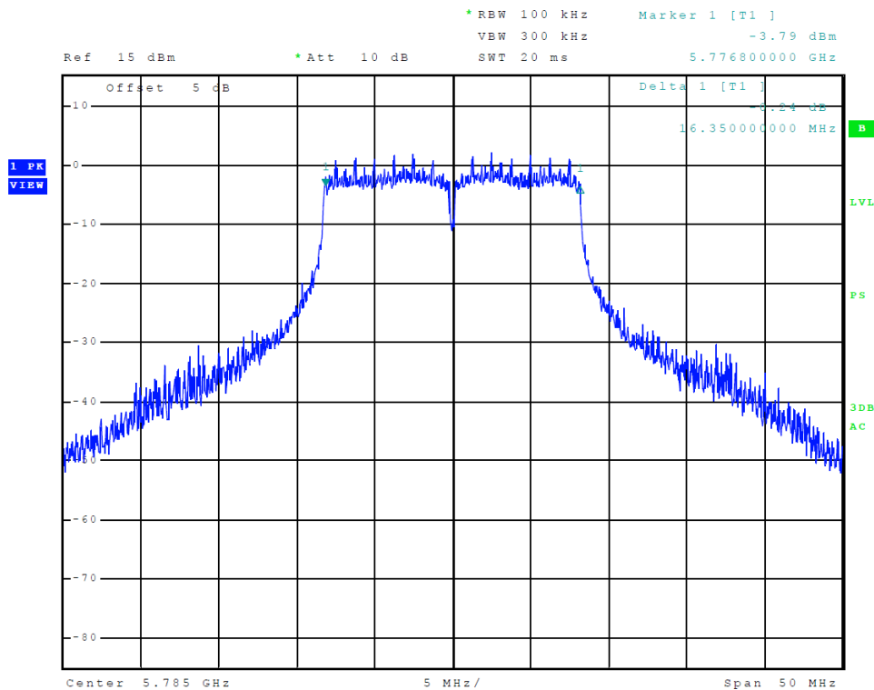
Figure 38 Plot of Transmitter Emissions (Chain 1, 5725-5850 MHz Band, 802.11a, 6-dB OBW)
