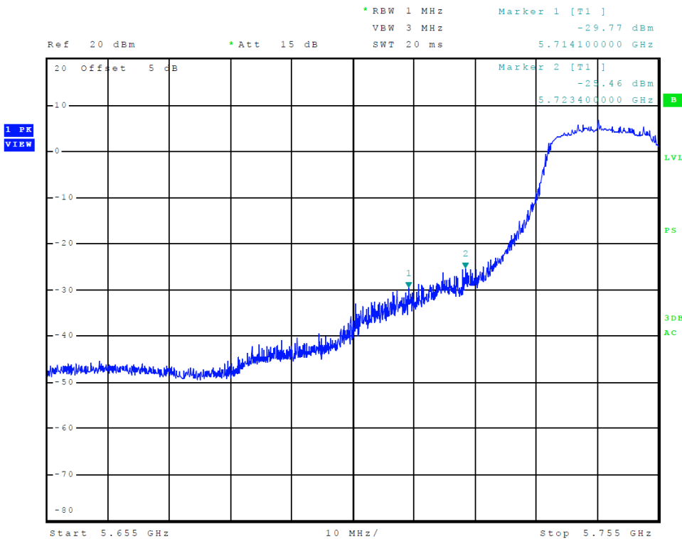
Figure 30 Plot of Transmitter Low Band Edge (Chain 1, 5725-5850 MHz Band, 802.11n40)
