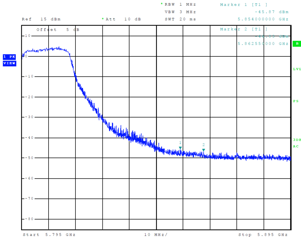
Figure 33 Plot of Transmitter High Band Edge (Chain 0, 5725-5850 MHz Band, 802.11n40)
