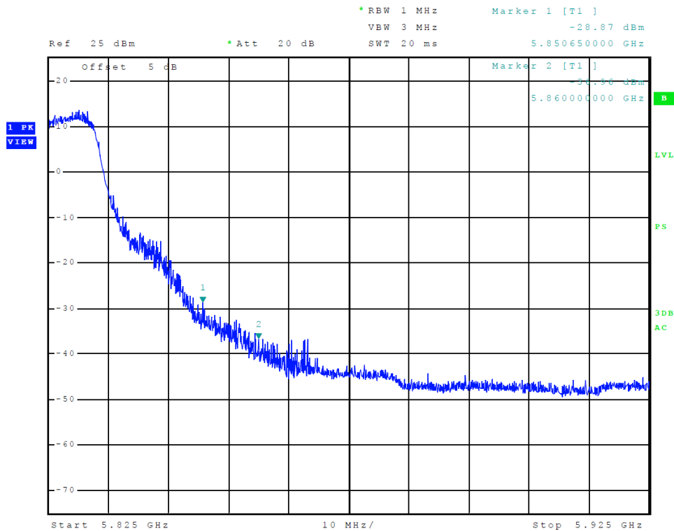
Figure 32 Plot of Transmitter High Band Edge (Chain 1, 5725-5850 MHz Band, 802.11a)
