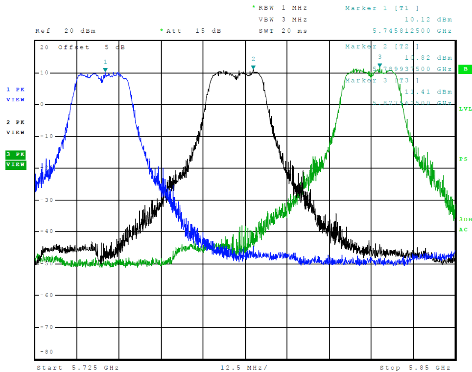
Figure 23 Plot of Transmitter Emissions (Chain 0, Across 5725-5850 MHz Band, 802.11a)
