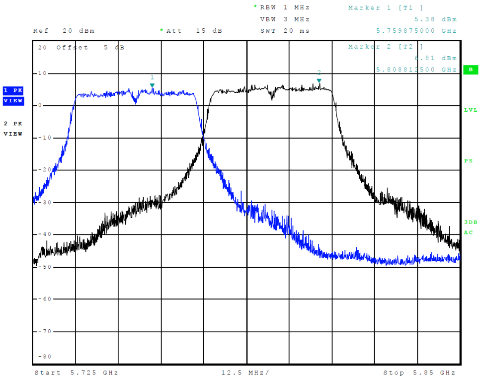
Figure 26 Plot of Transmitter Emissions (Chain 1, Across 5725-5850 MHz Band, 802.11n40)
