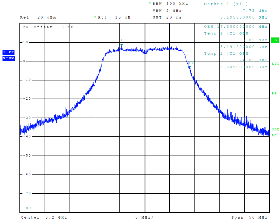
Figure 15 Plot of Transmitter Emissions (Chain 0, 5150-5250 MHz Band, 802.11a, 99% OBW)
