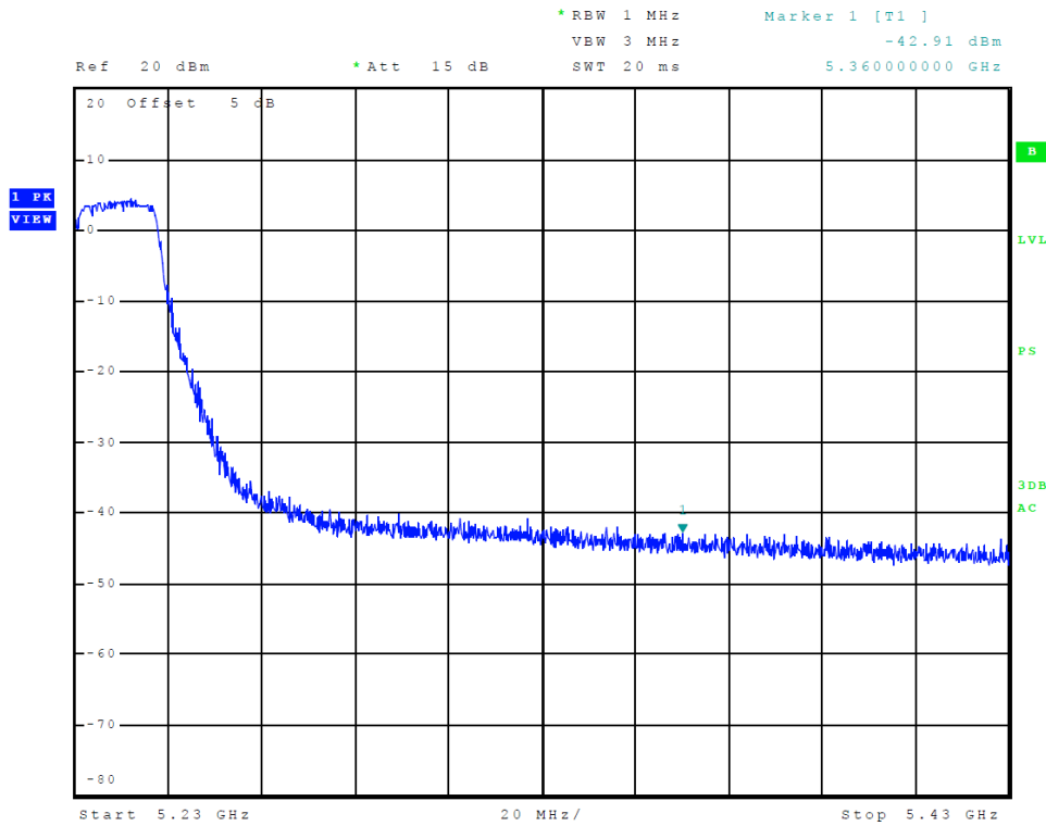
Figure 13 Plot of Transmitter High Band Edge (Chain 0, 5150-5250 MHz Band, 802.11n40)
