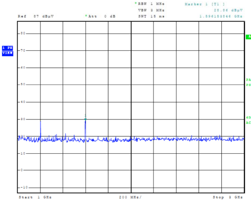
Figure Five General Radiated Emissions taken at 1 meter in screen room
